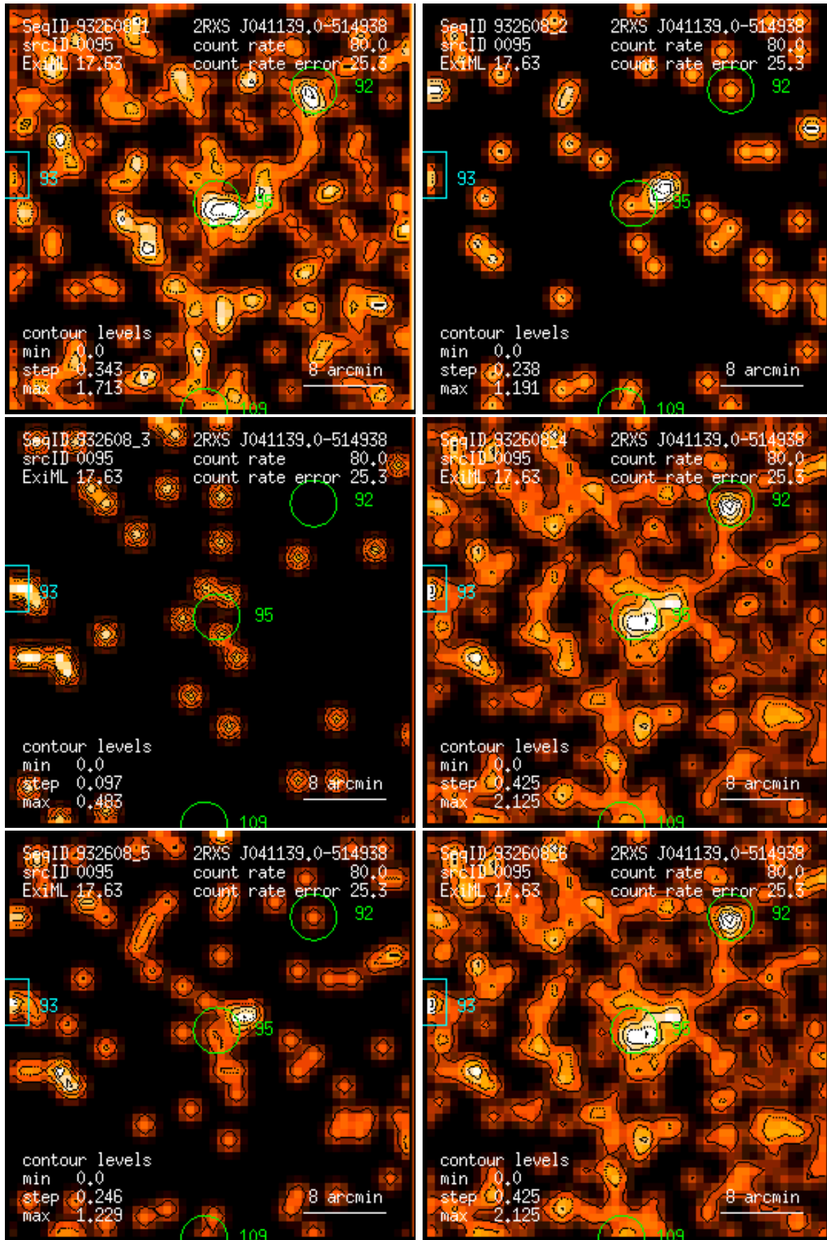
Figure 95: RASS 932608: detection 0095: band rate images, Gaussian filter: (1) PSPC channels 11 – 41, (2) 52 – 90, (3) 91 – 201, (4) 11 – 235, (5) 52 – 201, (6) 11 – 201. Broad band rates in counts/ks. Band rate contour levels in counts/ks/arcmin 2 .
