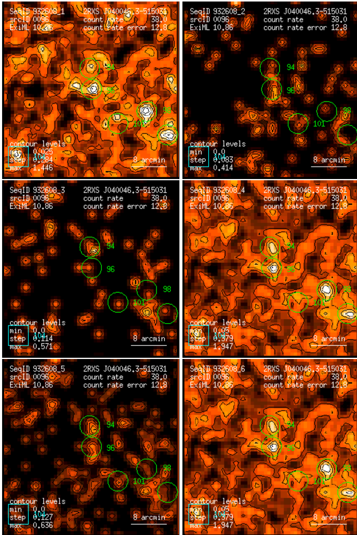
Figure 96: RASS 932608: detection 0096: band rate images, Gaussian filter: (1) PSPC channels 11 – 41, (2) 52 – 90, (3) 91 – 201, (4) 11 – 235, (5) 52 – 201, (6) 11 – 201. Broad band rates in counts/ks. Band rate contour levels in counts/ks/arcmin 2 .
