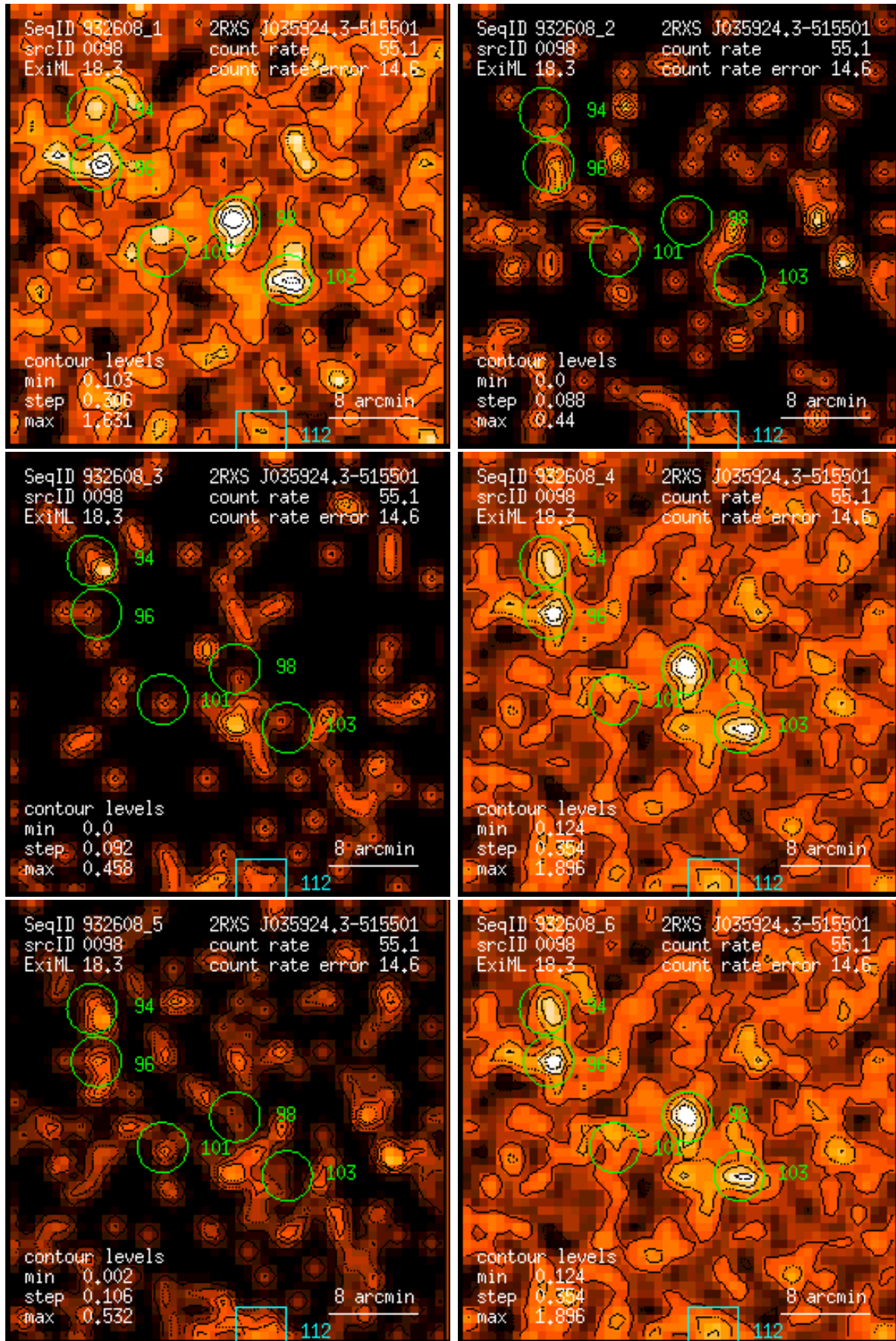
Figure 98: RASS 932608: detection 0098: band rate images, Gaussian filter: (1) PSPC channels 11 – 41, (2) 52 – 90, (3) 91 – 201, (4) 11 – 235, (5) 52 – 201, (6) 11 – 201. Broad band rates in counts/ks. Band rate contour levels in counts/ks/arcmin 2 .
