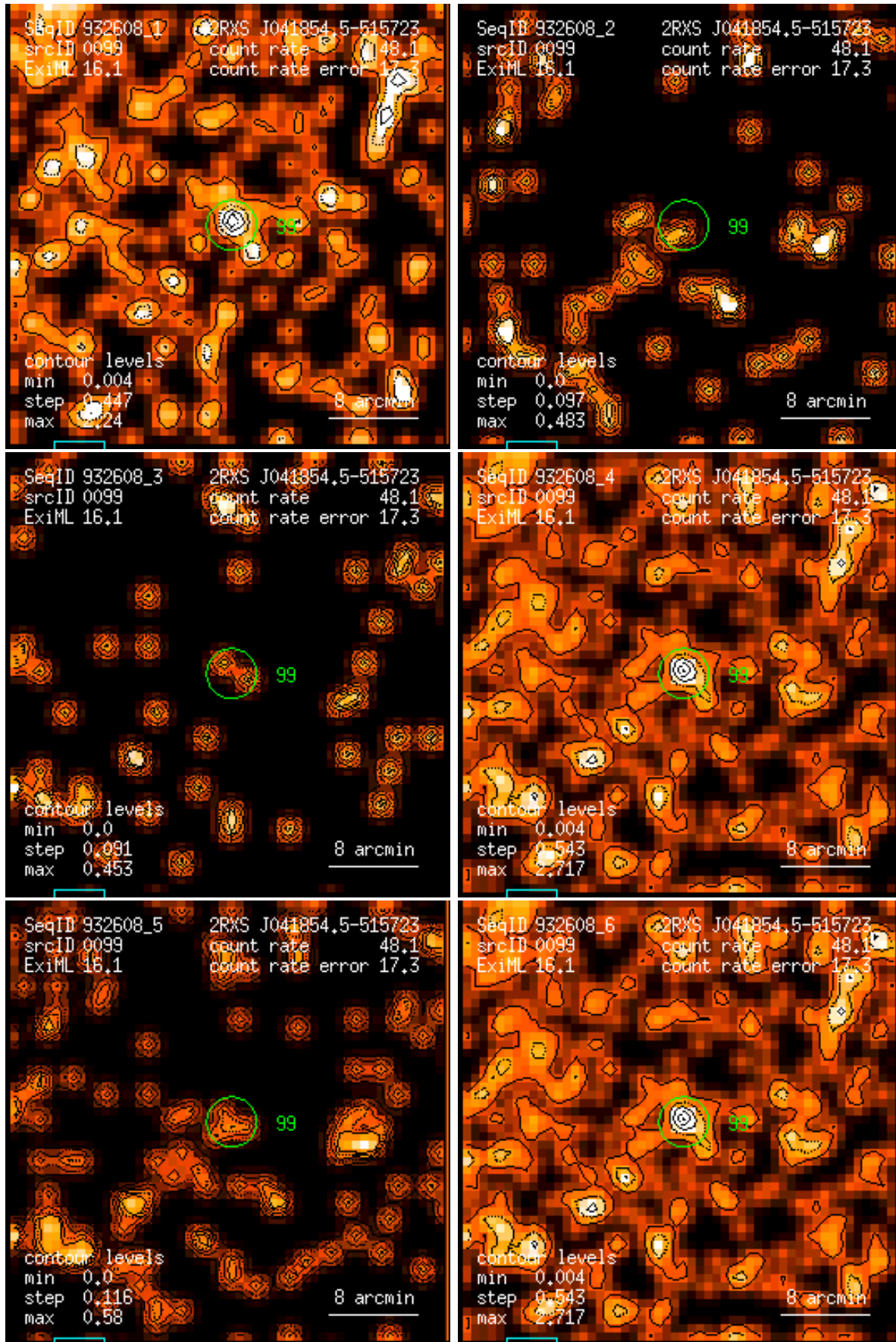
Figure 99: RASS 932608: detection 0099: band rate images, Gaussian filter: (1) PSPC channels 11 – 41, (2) 52 – 90, (3) 91 – 201, (4) 11 – 235, (5) 52 – 201, (6) 11 – 201. Broad band rates in counts/ks. Band rate contour levels in counts/ks/arcmin 2 .
