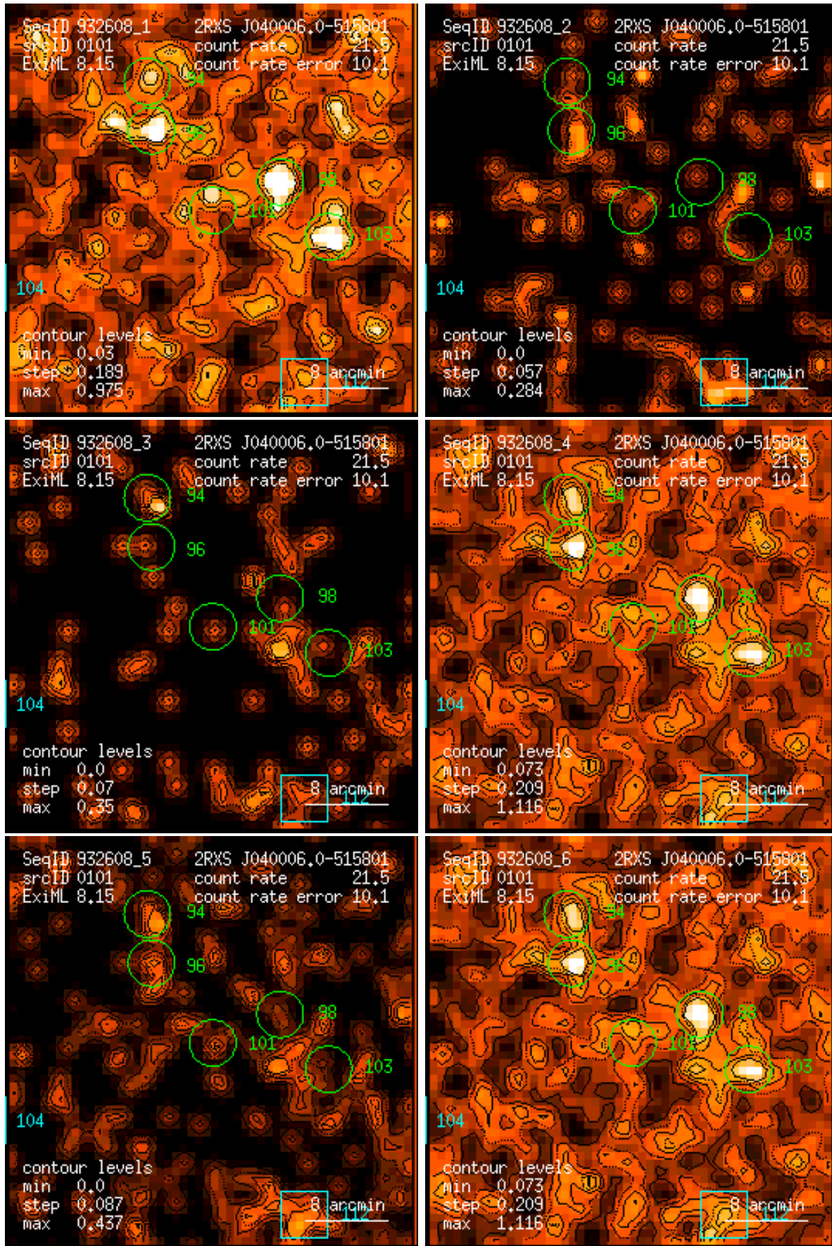
Figure 101: RASS 932608: detection 0101: band rate images, Gaussian filter: (1) PSPC channels 11 – 41, (2) 52 – 90, (3) 91 – 201, (4) 11 – 235, (5) 52 – 201, (6) 11 – 201. Broad band rates in counts/ks. Band rate contour levels in counts/ks/arcmin 2 .
