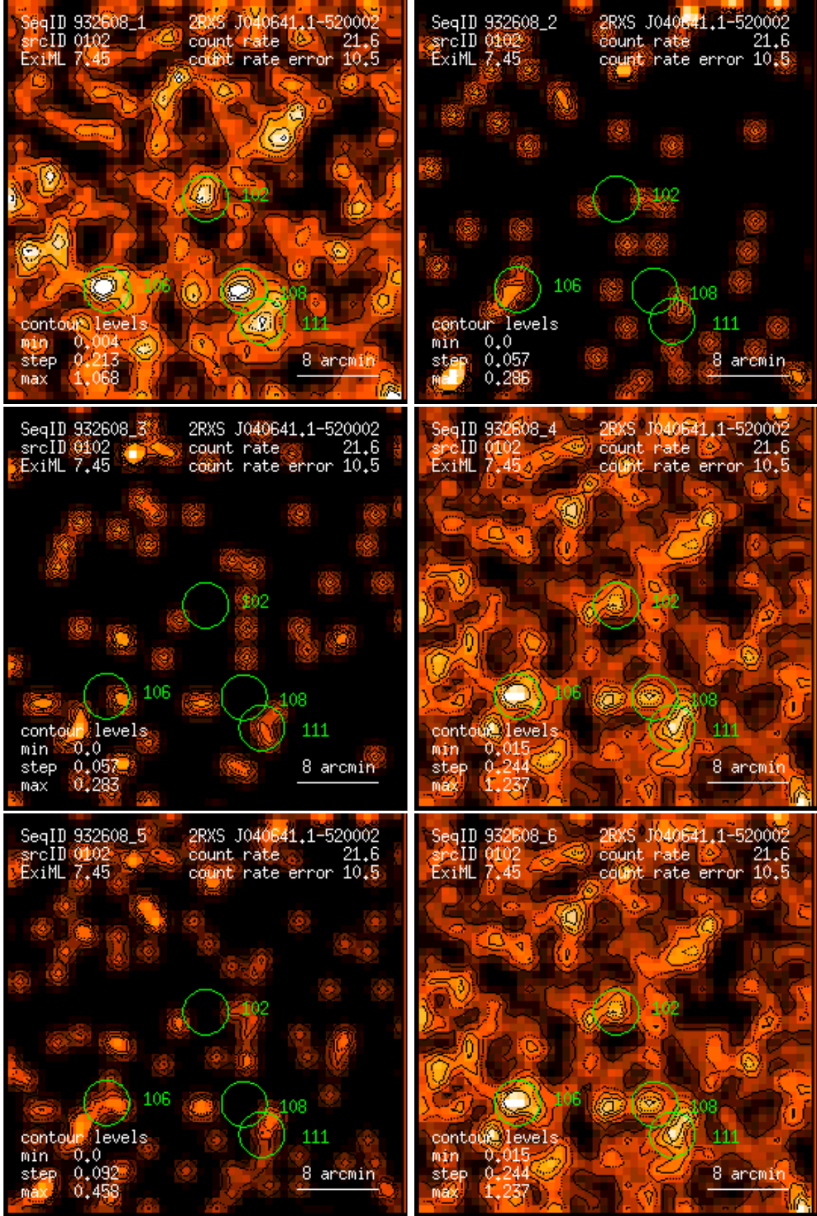
Figure 102: RASS 932608: detection 0102: band rate images, Gaussian filter: (1) PSPC channels 11 – 41, (2) 52 – 90, (3) 91 – 201, (4) 11 – 235, (5) 52 – 201, (6) 11 – 201. Broad band rates in counts/ks. Band rate contour levels in counts/ks/arcmin 2 .
