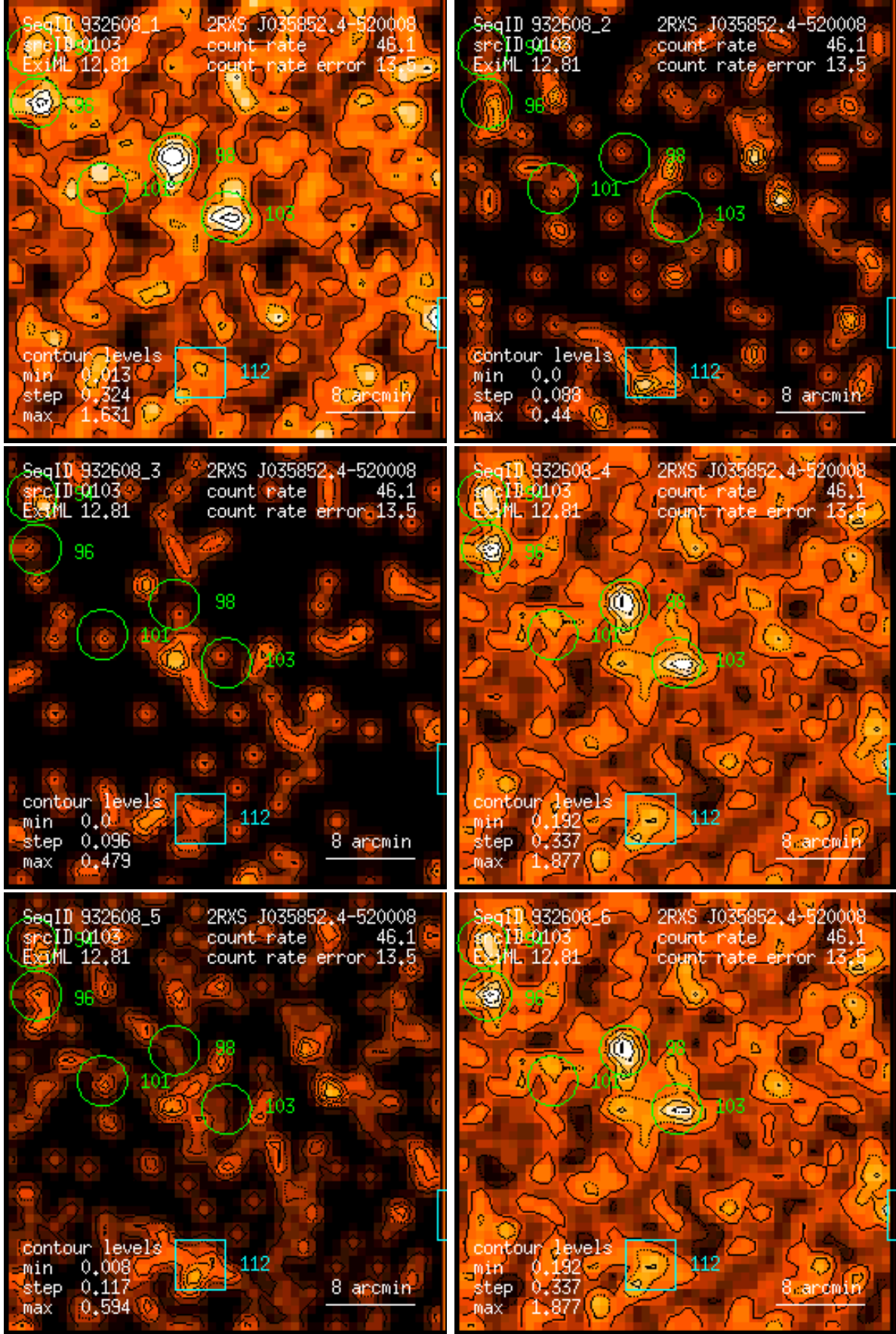
Figure 103: RASS 932608: detection 0103: band rate images, Gaussian filter: (1) PSPC channels 11 – 41, (2) 52 – 90, (3) 91 – 201, (4) 11 – 235, (5) 52 – 201, (6) 11 – 201. Broad band rates in counts/ks. Band rate contour levels in counts/ks/arcmin 2 .
