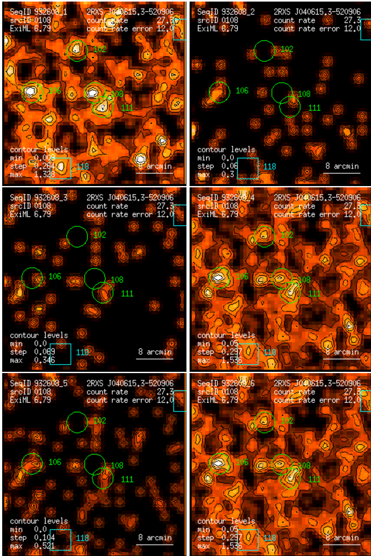
Figure 108: RASS 932608: detection 0108: band rate images, Gaussian filter: (1) PSPC channels 11 – 41, (2) 52 – 90, (3) 91 – 201, (4) 11 – 235, (5) 52 – 201, (6) 11 – 201. Broad band rates in counts/ks. Band rate contour levels in counts/ks/arcmin 2 .
