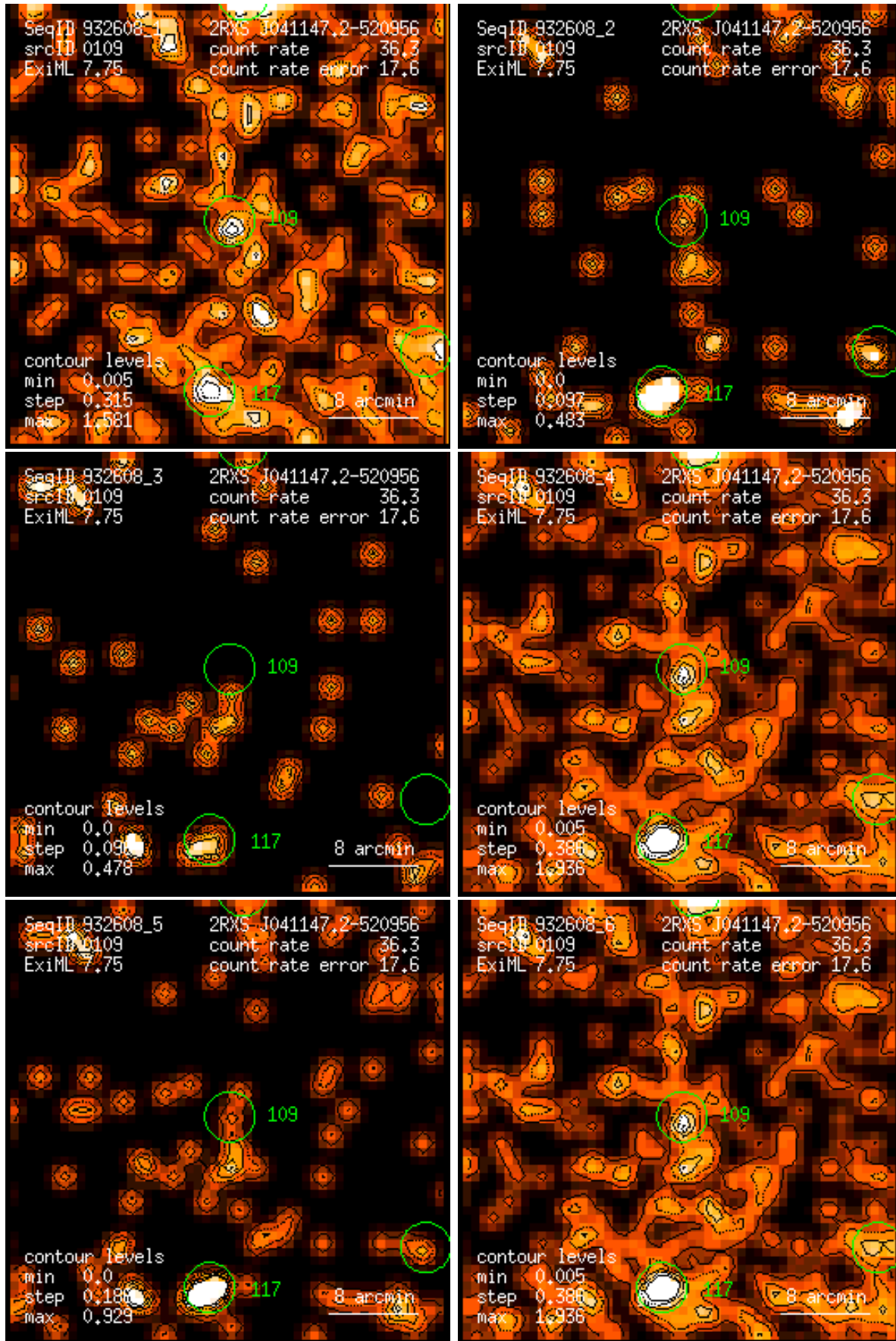
Figure 109: RASS 932608: detection 0109: band rate images, Gaussian filter: (1) PSPC channels 11 – 41, (2) 52 – 90, (3) 91 – 201, (4) 11 – 235, (5) 52 – 201, (6) 11 – 201. Broad band rates in counts/ks. Band rate contour levels in counts/ks/arcmin 2 .
