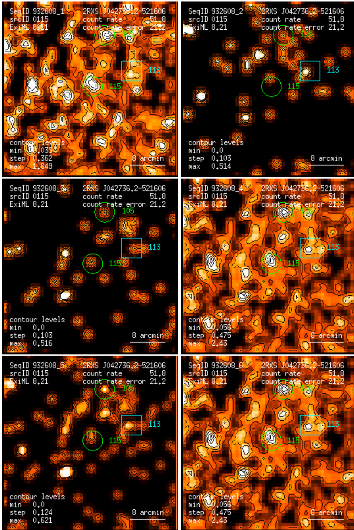
Figure 115: RASS 932608: detection 0115: band rate images, Gaussian filter: (1) PSPC channels 11 – 41, (2) 52 – 90, (3) 91 – 201, (4) 11 – 235, (5) 52 – 201, (6) 11 – 201. Broad band rates in counts/ks. Band rate contour levels in counts/ks/arcmin 2 .
