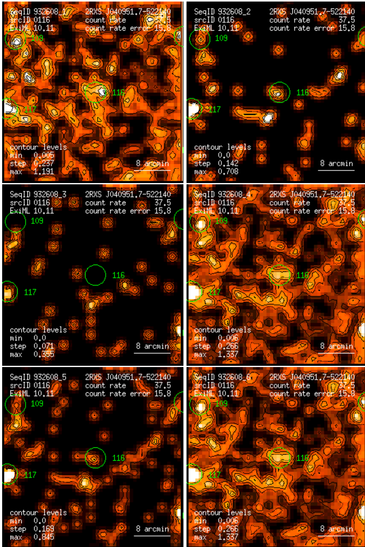
Figure 116: RASS 932608: detection 0116: band rate images, Gaussian filter: (1) PSPC channels 11 – 41, (2) 52 – 90, (3) 91 – 201, (4) 11 – 235, (5) 52 – 201, (6) 11 – 201. Broad band rates in counts/ks. Band rate contour levels in counts/ks/arcmin 2 .
