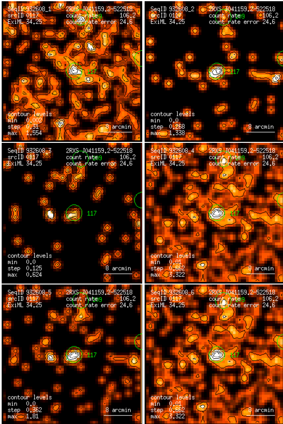
Figure 117: RASS 932608: detection 0117: band rate images, Gaussian filter: (1) PSPC channels 11 – 41, (2) 52 – 90, (3) 91 – 201, (4) 11 – 235, (5) 52 – 201, (6) 11 – 201. Broad band rates in counts/ks. Band rate contour levels in counts/ks/arcmin 2 .
