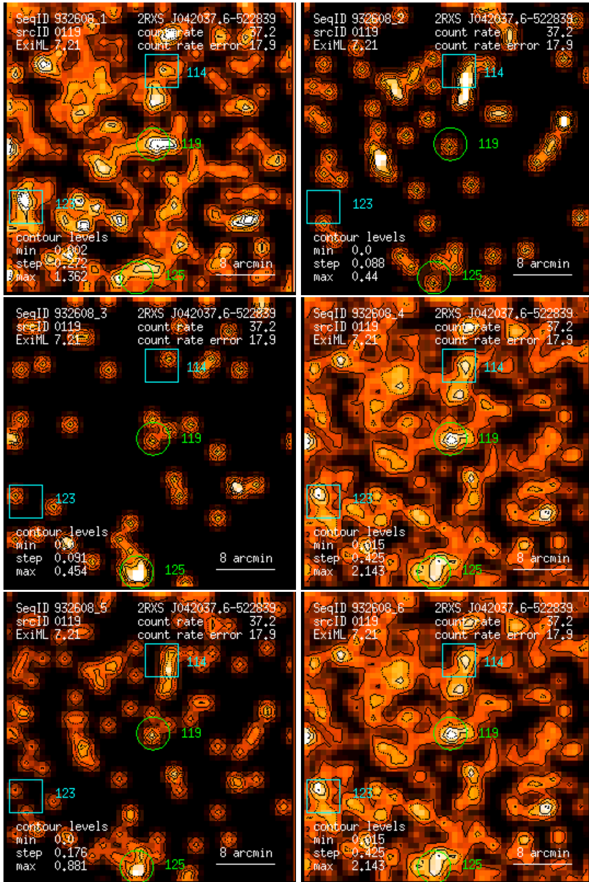
Figure 119: RASS 932608: detection 0119: band rate images, Gaussian filter: (1) PSPC channels 11 – 41, (2) 52 – 90, (3) 91 – 201, (4) 11 – 235, (5) 52 – 201, (6) 11 – 201. Broad band rates in counts/ks. Band rate contour levels in counts/ks/arcmin 2 .
