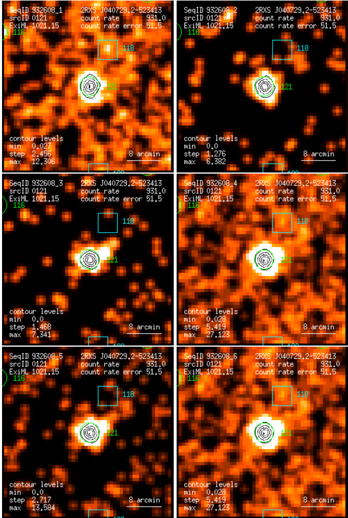
Figure 121: RASS 932608: detection 0121: band rate images, Gaussian filter: (1) PSPC channels 11 – 41, (2) 52 – 90, (3) 91 – 201, (4) 11 – 235, (5) 52 – 201, (6) 11 – 201. Broad band rates in counts/ks. Band rate contour levels in counts/ks/arcmin 2 .
