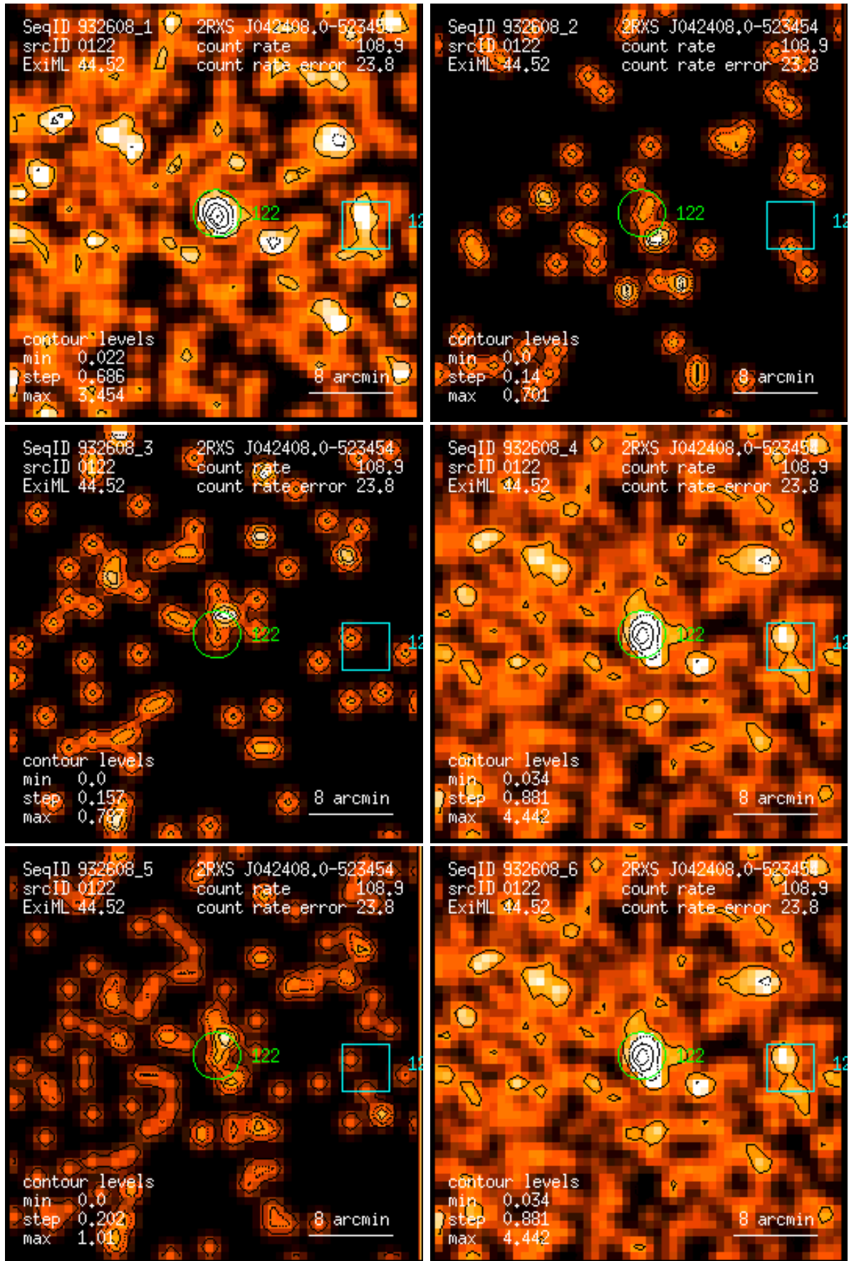
Figure 122: RASS 932608: detection 0122: band rate images, Gaussian filter: (1) PSPC channels 11 – 41, (2) 52 – 90, (3) 91 – 201, (4) 11 – 235, (5) 52 – 201, (6) 11 – 201. Broad band rates in counts/ks. Band rate contour levels in counts/ks/arcmin 2 .
