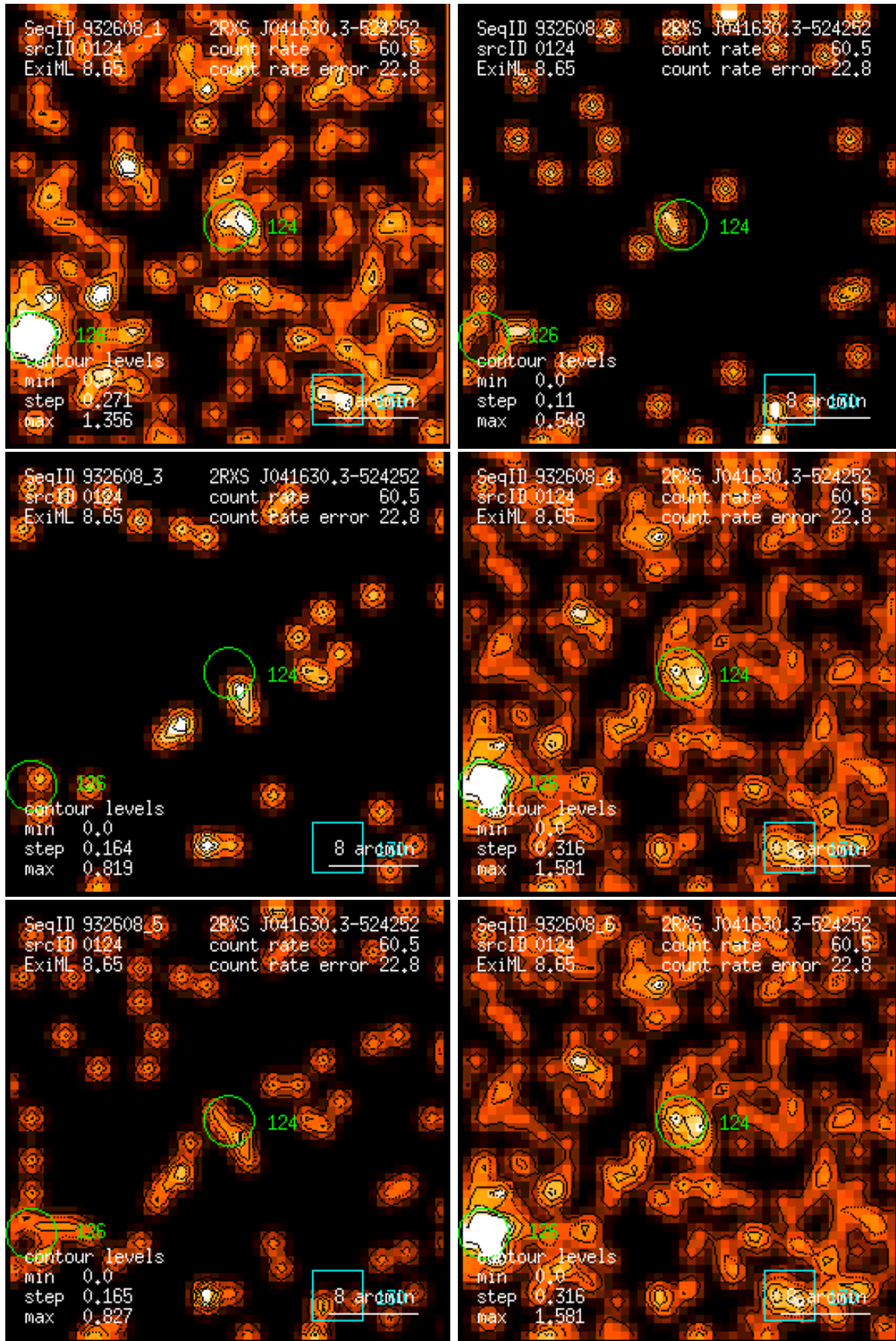
Figure 124: RASS 932608: detection 0124: band rate images, Gaussian filter: (1) PSPC channels 11 – 41, (2) 52 – 90, (3) 91 – 201, (4) 11 – 235, (5) 52 – 201, (6) 11 – 201. Broad band rates in counts/ks. Band rate contour levels in counts/ks/arcmin 2 .
