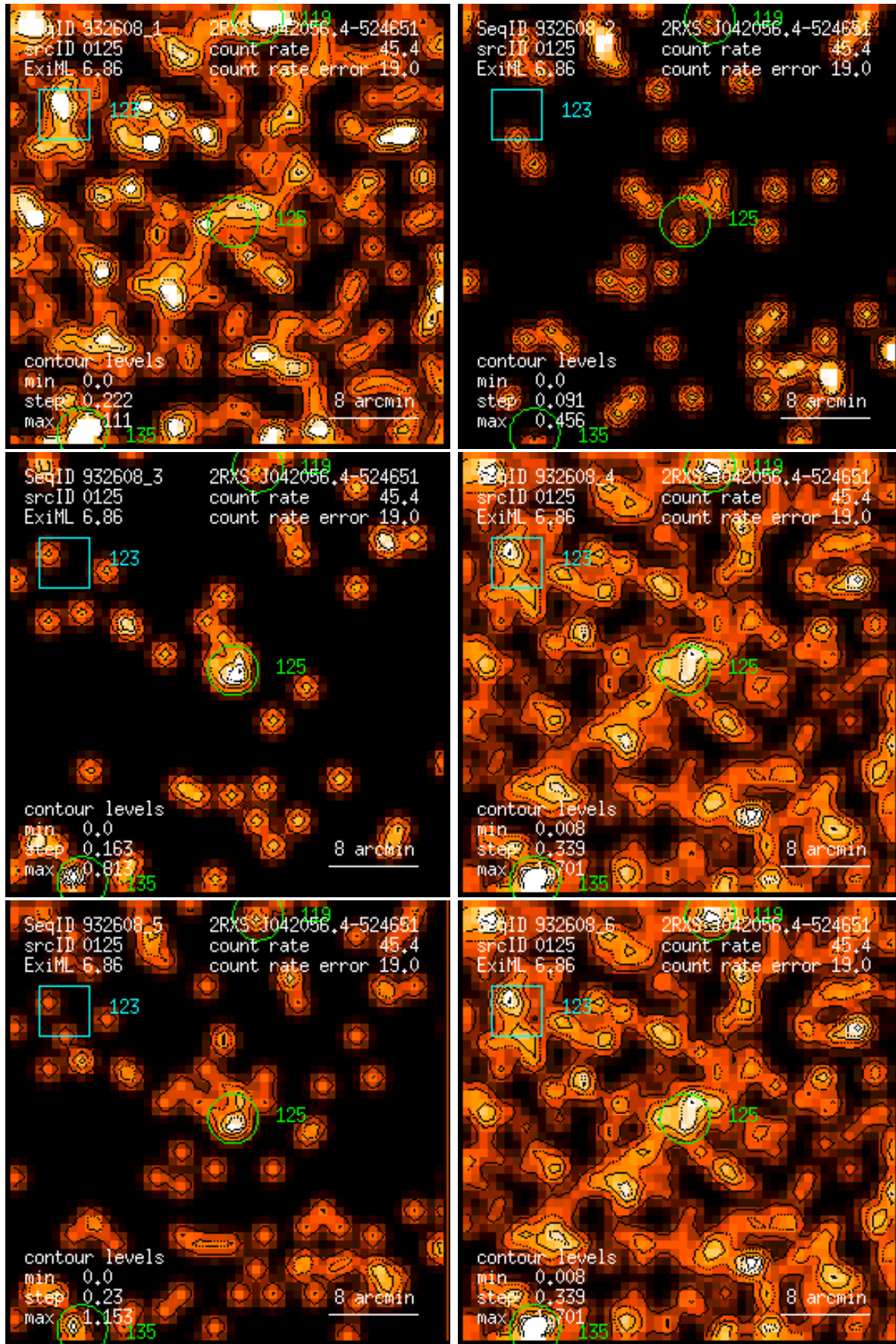
Figure 125: RASS 932608: detection 0125: band rate images, Gaussian filter: (1) PSPC channels 11 – 41, (2) 52 – 90, (3) 91 – 201, (4) 11 – 235, (5) 52 – 201, (6) 11 – 201. Broad band rates in counts/ks. Band rate contour levels in counts/ks/arcmin 2 .
