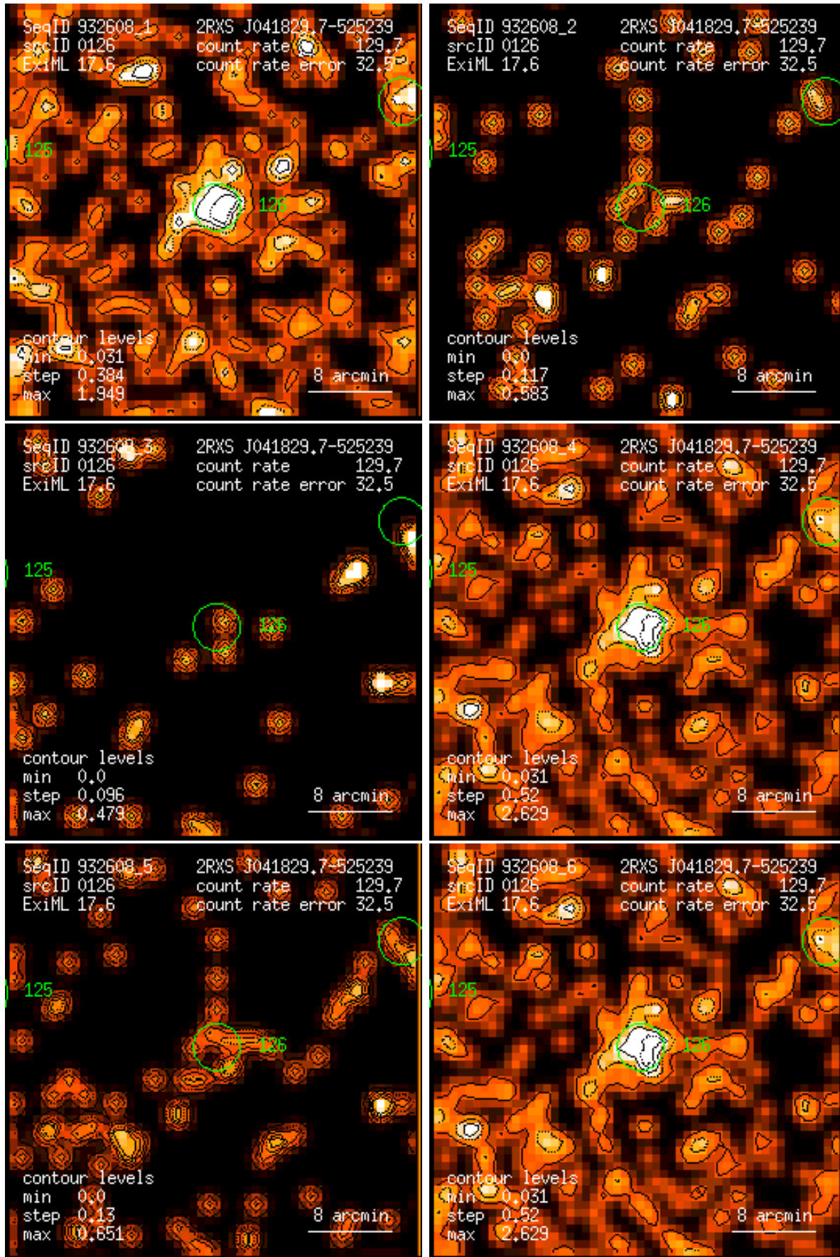
Figure 126: RASS 932608: detection 0126: band rate images, Gaussian filter: (1) PSPC channels 11 – 41, (2) 52 – 90, (3) 91 – 201, (4) 11 – 235, (5) 52 – 201, (6) 11 – 201. Broad band rates in counts/ks. Band rate contour levels in counts/ks/arcmin 2 .
