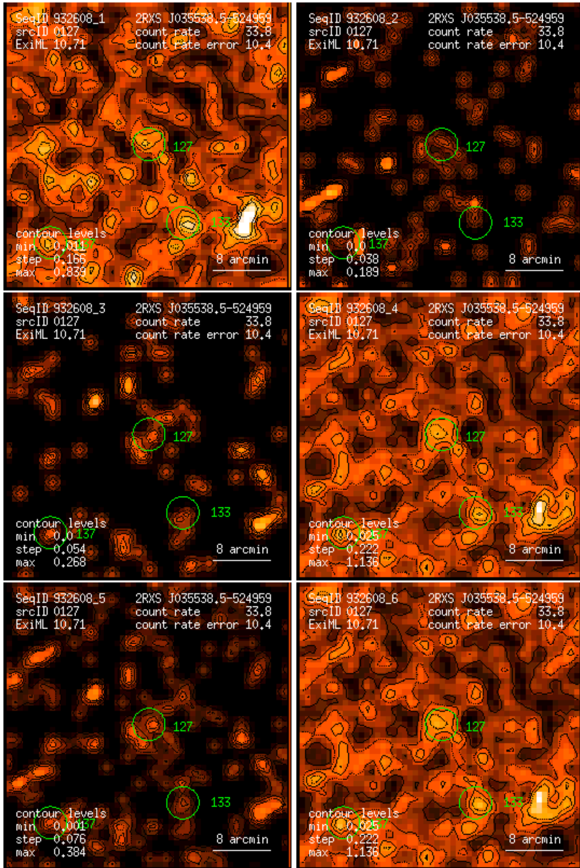
Figure 127: RASS 932608: detection 0127: band rate images, Gaussian filter: (1) PSPC channels 11 – 41, (2) 52 – 90, (3) 91 – 201, (4) 11 – 235, (5) 52 – 201, (6) 11 – 201. Broad band rates in counts/ks. Band rate contour levels in counts/ks/arcmin 2 .
