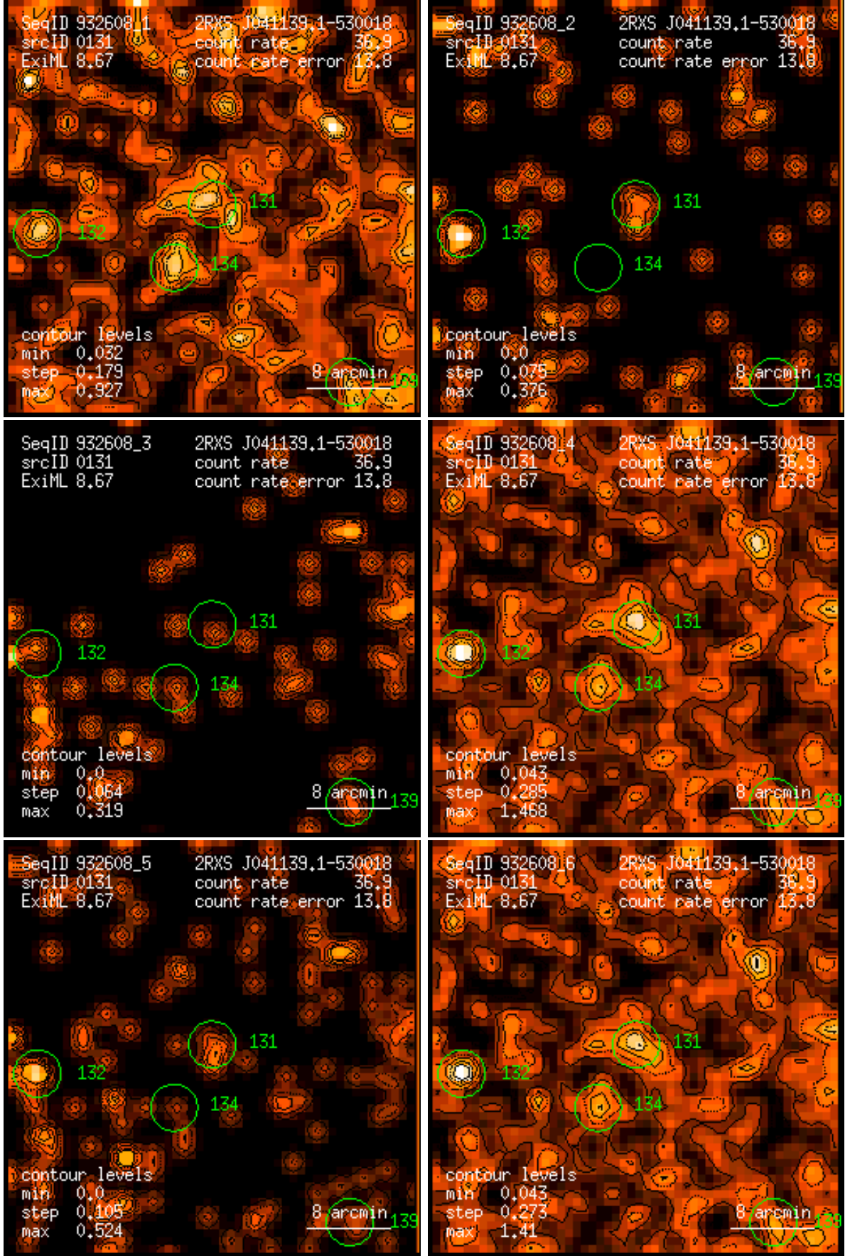
Figure 131: RASS 932608: detection 0131: band rate images, Gaussian filter: (1) PSPC channels 11 – 41, (2) 52 – 90, (3) 91 – 201, (4) 11 – 235, (5) 52 – 201, (6) 11 – 201. Broad band rates in counts/ks. Band rate contour levels in counts/ks/arcmin 2 .
