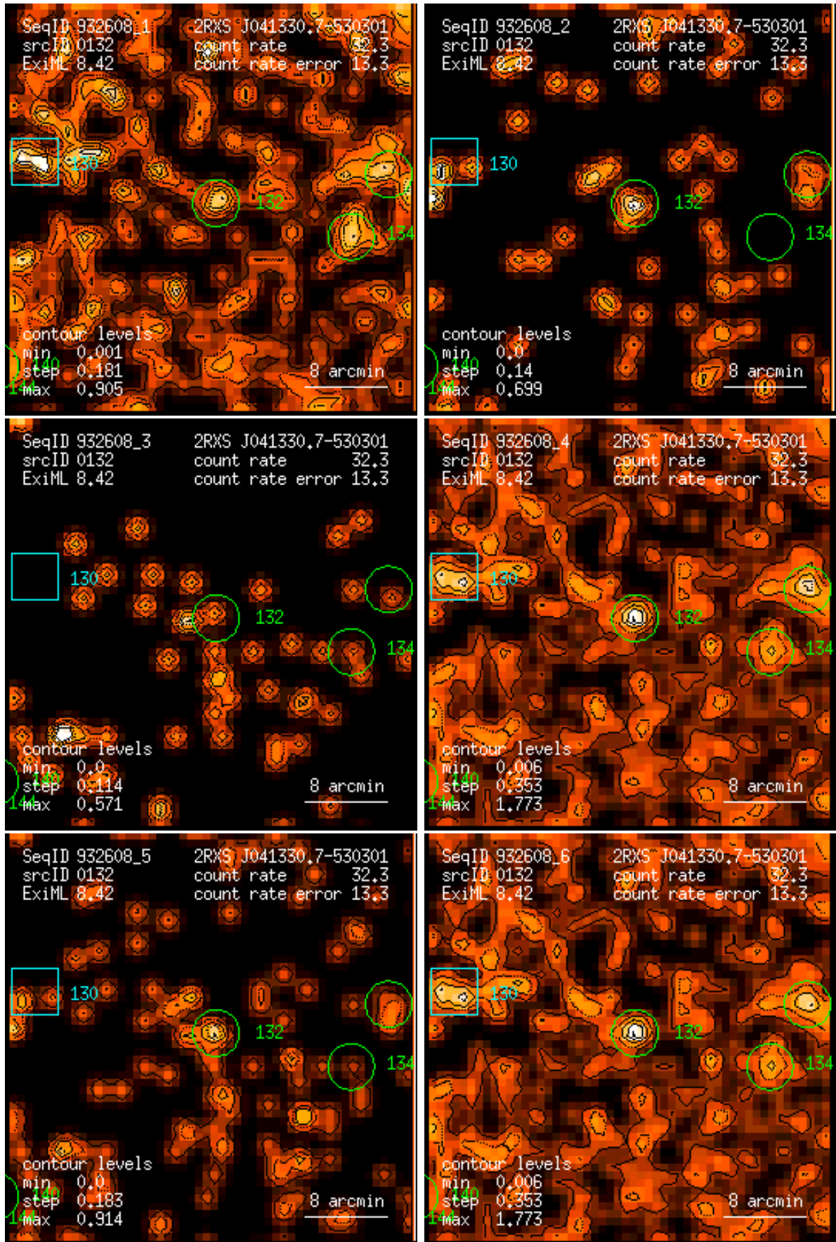
Figure 132: RASS 932608: detection 0132: band rate images, Gaussian filter: (1) PSPC channels 11 – 41, (2) 52 – 90, (3) 91 – 201, (4) 11 – 235, (5) 52 – 201, (6) 11 – 201. Broad band rates in counts/ks. Band rate contour levels in counts/ks/arcmin 2 .
