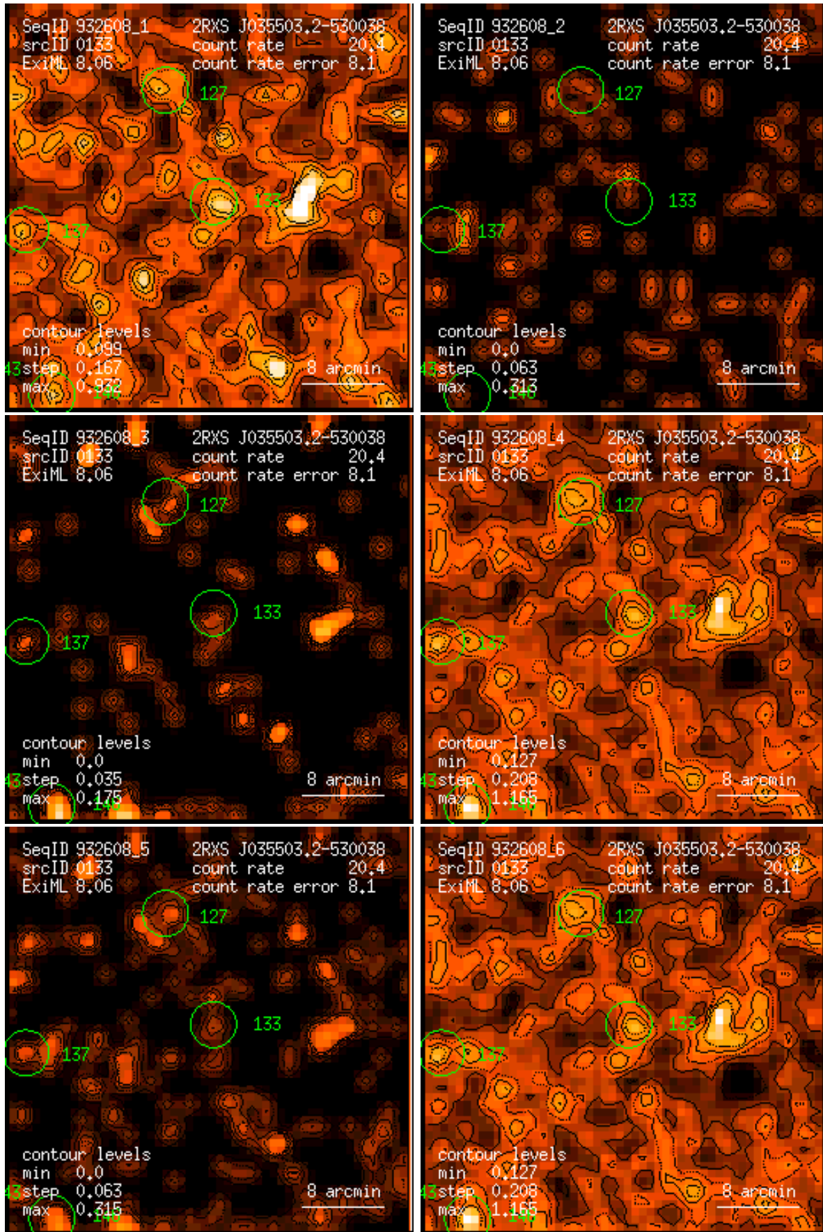
Figure 133: RASS 932608: detection 0133: band rate images, Gaussian filter: (1) PSPC channels 11 – 41, (2) 52 – 90, (3) 91 – 201, (4) 11 – 235, (5) 52 – 201, (6) 11 – 201. Broad band rates in counts/ks. Band rate contour levels in counts/ks/arcmin 2 .
