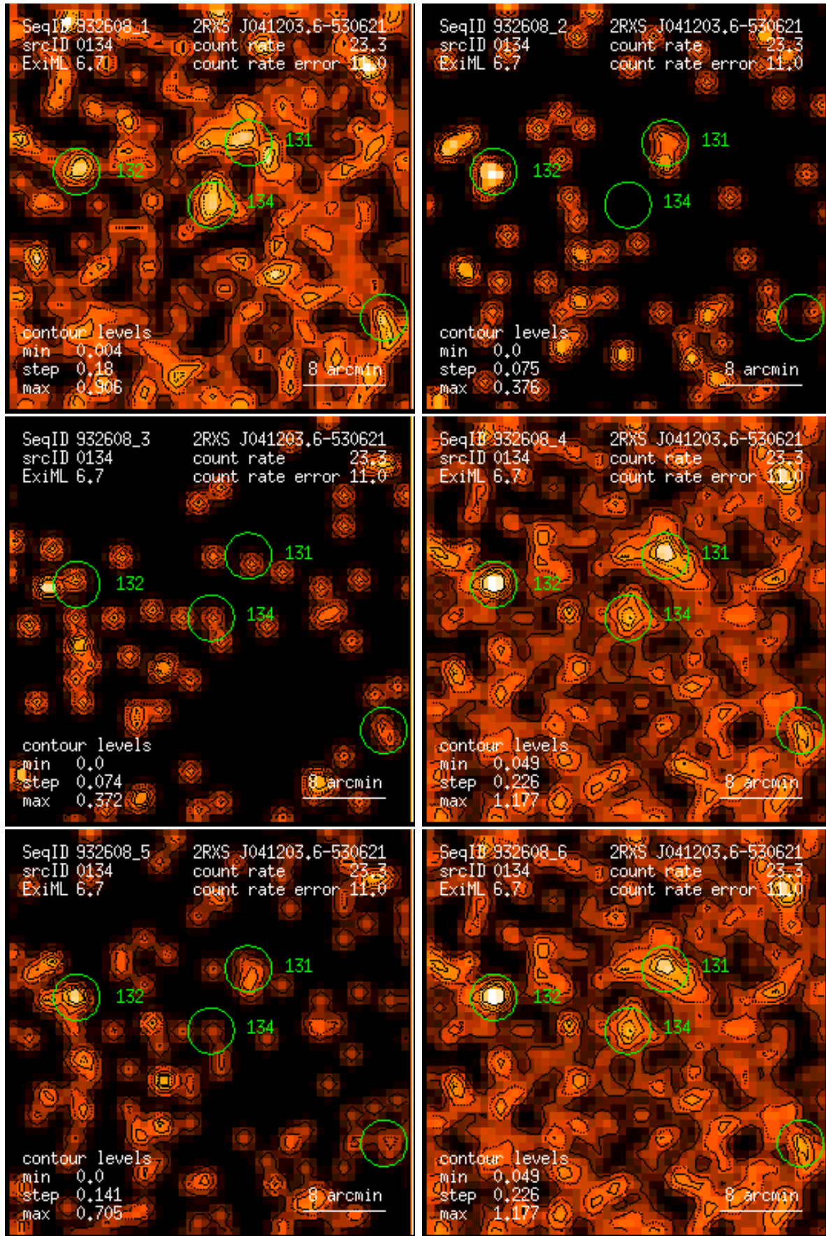
Figure 134: RASS 932608: detection 0134: band rate images, Gaussian filter: (1) PSPC channels 11 – 41, (2) 52 – 90, (3) 91 – 201, (4) 11 – 235, (5) 52 – 201, (6) 11 – 201. Broad band rates in counts/ks. Band rate contour levels in counts/ks/arcmin 2 .
