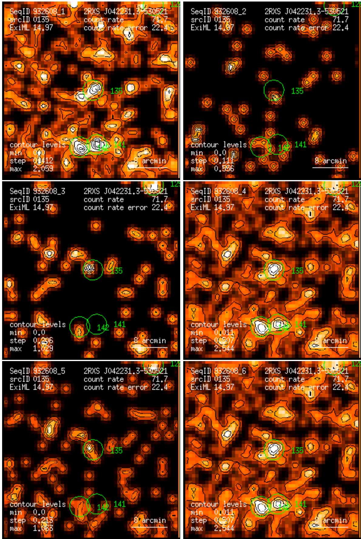
Figure 135: RASS 932608: detection 0135: band rate images, Gaussian filter: (1) PSPC channels 11 – 41, (2) 52 – 90, (3) 91 – 201, (4) 11 – 235, (5) 52 – 201, (6) 11 – 201. Broad band rates in counts/ks. Band rate contour levels in counts/ks/arcmin 2 .
