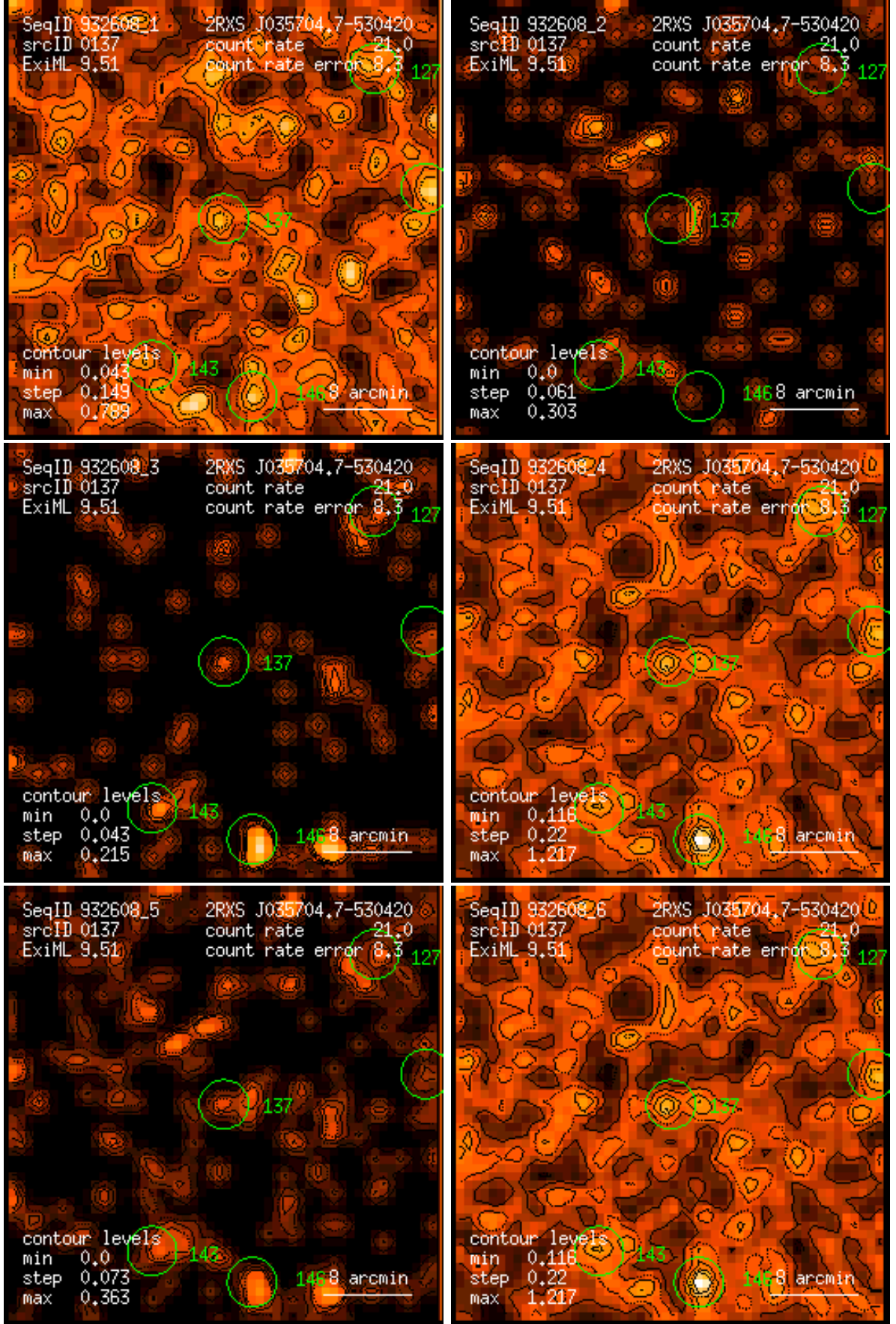
Figure 137: RASS 932608: detection 0137: band rate images, Gaussian filter: (1) PSPC channels 11 – 41, (2) 52 – 90, (3) 91 – 201, (4) 11 – 235, (5) 52 – 201, (6) 11 – 201. Broad band rates in counts/ks. Band rate contour levels in counts/ks/arcmin 2 .
