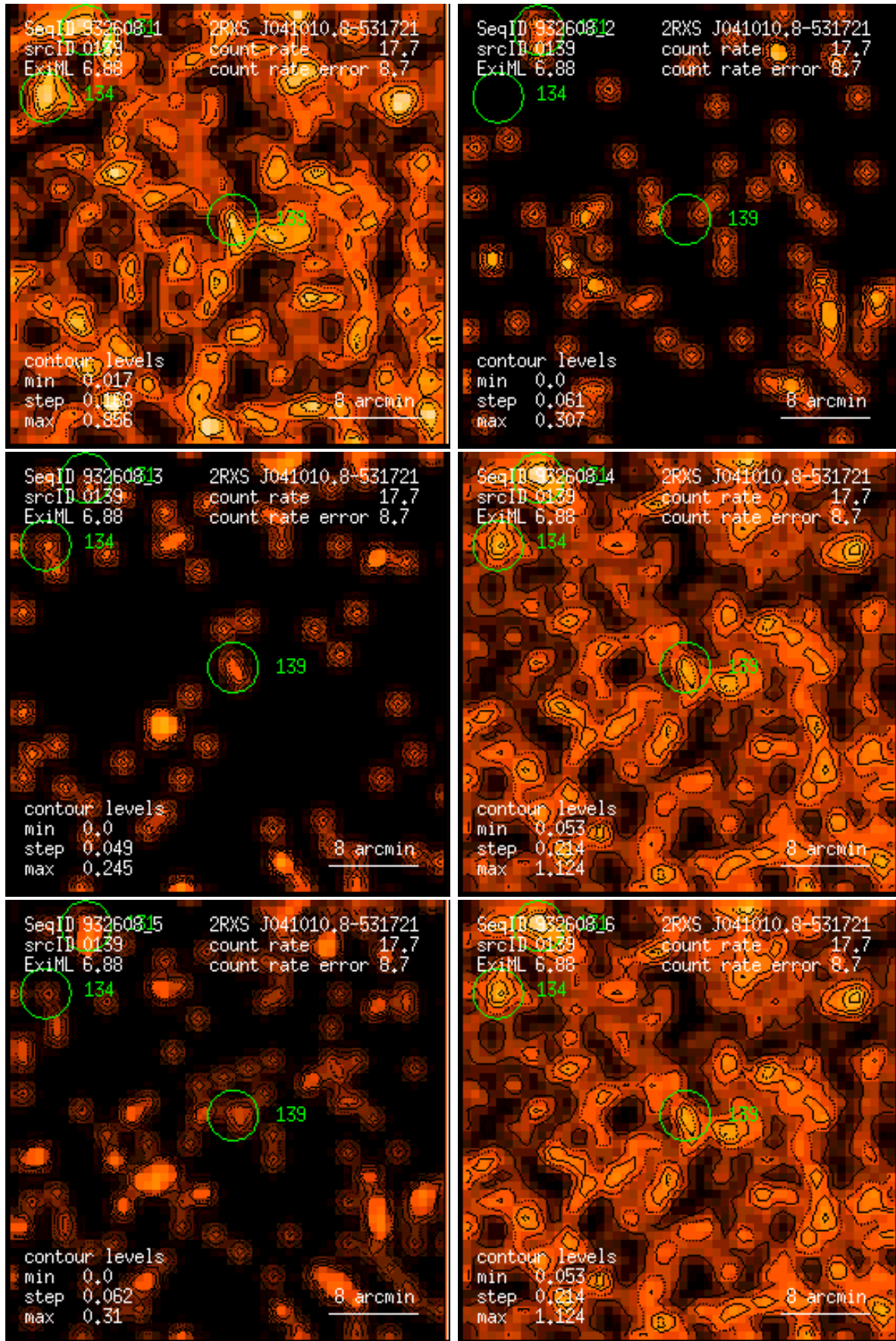
Figure 139: RASS 932608: detection 0139: band rate images, Gaussian filter: (1) PSPC channels 11 – 41, (2) 52 – 90, (3) 91 – 201, (4) 11 – 235, (5) 52 – 201, (6) 11 – 201. Broad band rates in counts/ks. Band rate contour levels in counts/ks/arcmin 2 .
