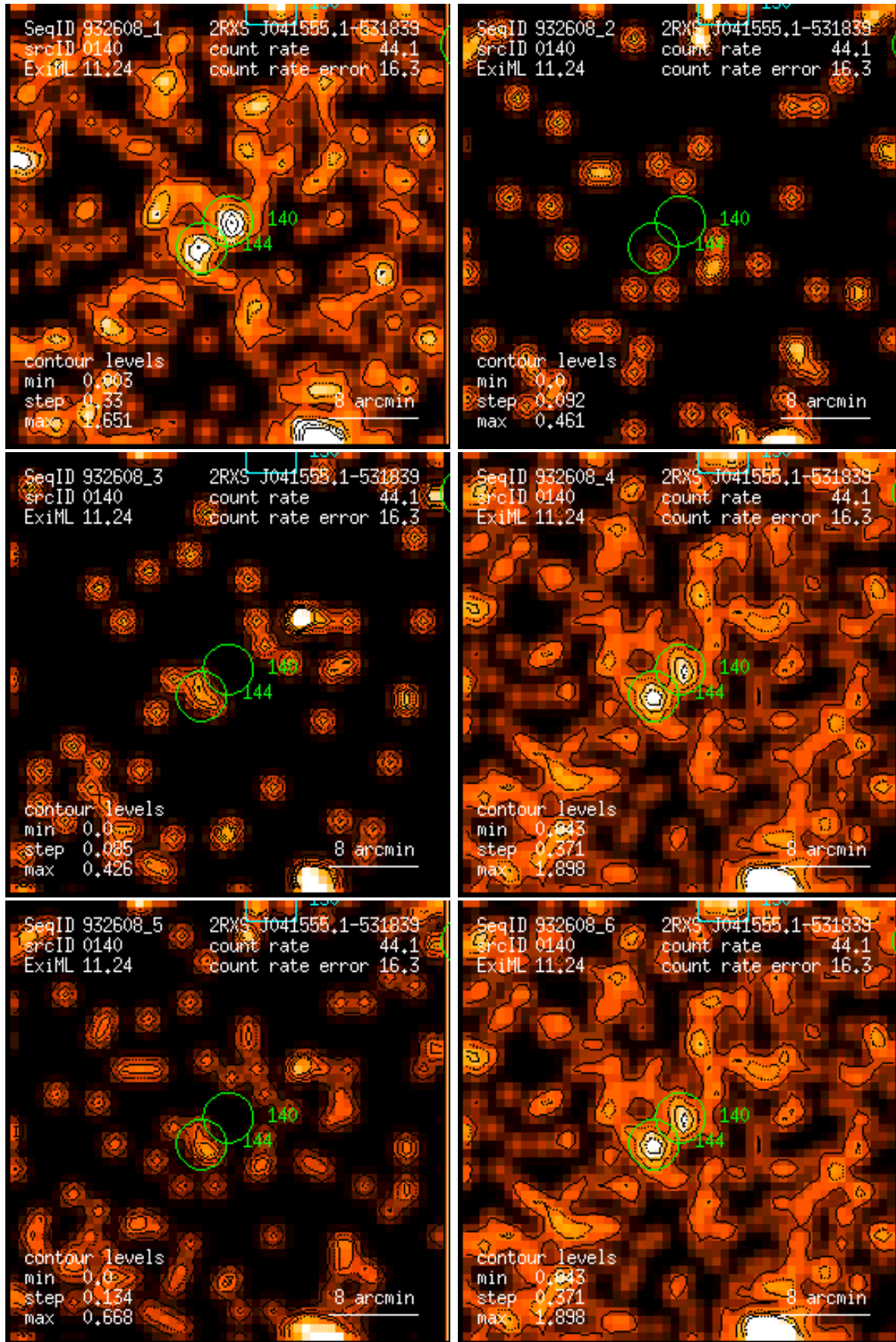
Figure 140: RASS 932608: detection 0140: band rate images, Gaussian filter: (1) PSPC channels 11 – 41, (2) 52 – 90, (3) 91 – 201, (4) 11 – 235, (5) 52 – 201, (6) 11 – 201. Broad band rates in counts/ks. Band rate contour levels in counts/ks/arcmin 2 .
