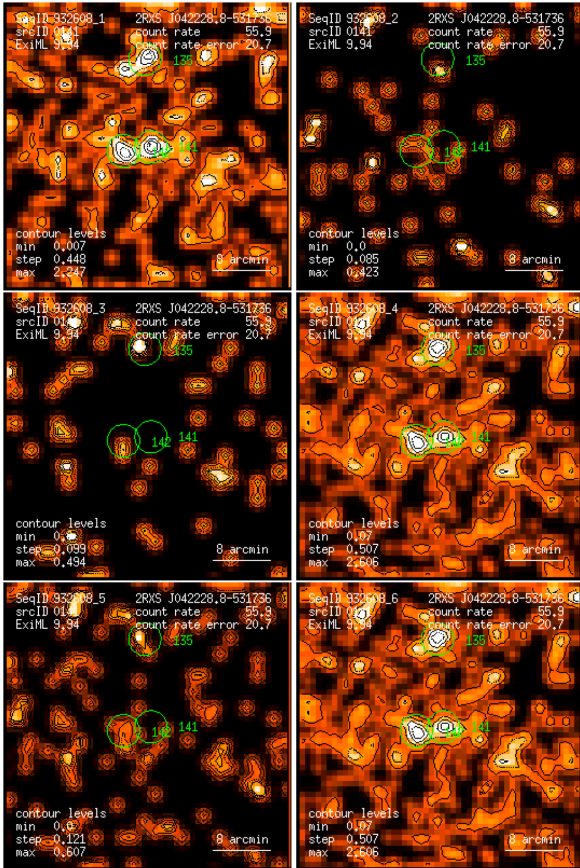
Figure 141: RASS 932608: detection 0141: band rate images, Gaussian filter: (1) PSPC channels 11 – 41, (2) 52 – 90, (3) 91 – 201, (4) 11 – 235, (5) 52 – 201, (6) 11 – 201. Broad band rates in counts/ks. Band rate contour levels in counts/ks/arcmin 2 .
