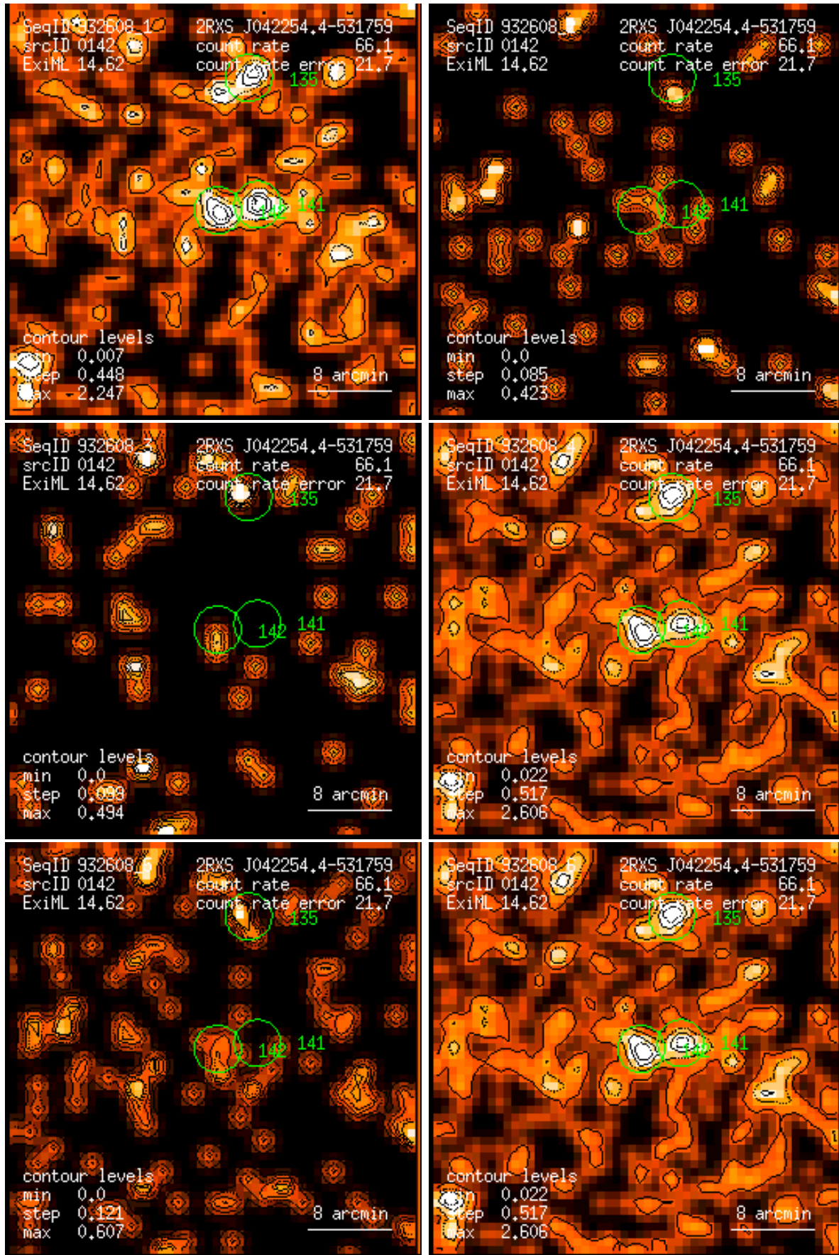
Figure 142: RASS 932608: detection 0142: band rate images, Gaussian filter: (1) PSPC channels 11 – 41, (2) 52 – 90, (3) 91 – 201, (4) 11 – 235, (5) 52 – 201, (6) 11 – 201. Broad band rates in counts/ks. Band rate contour levels in counts/ks/arcmin 2 .
