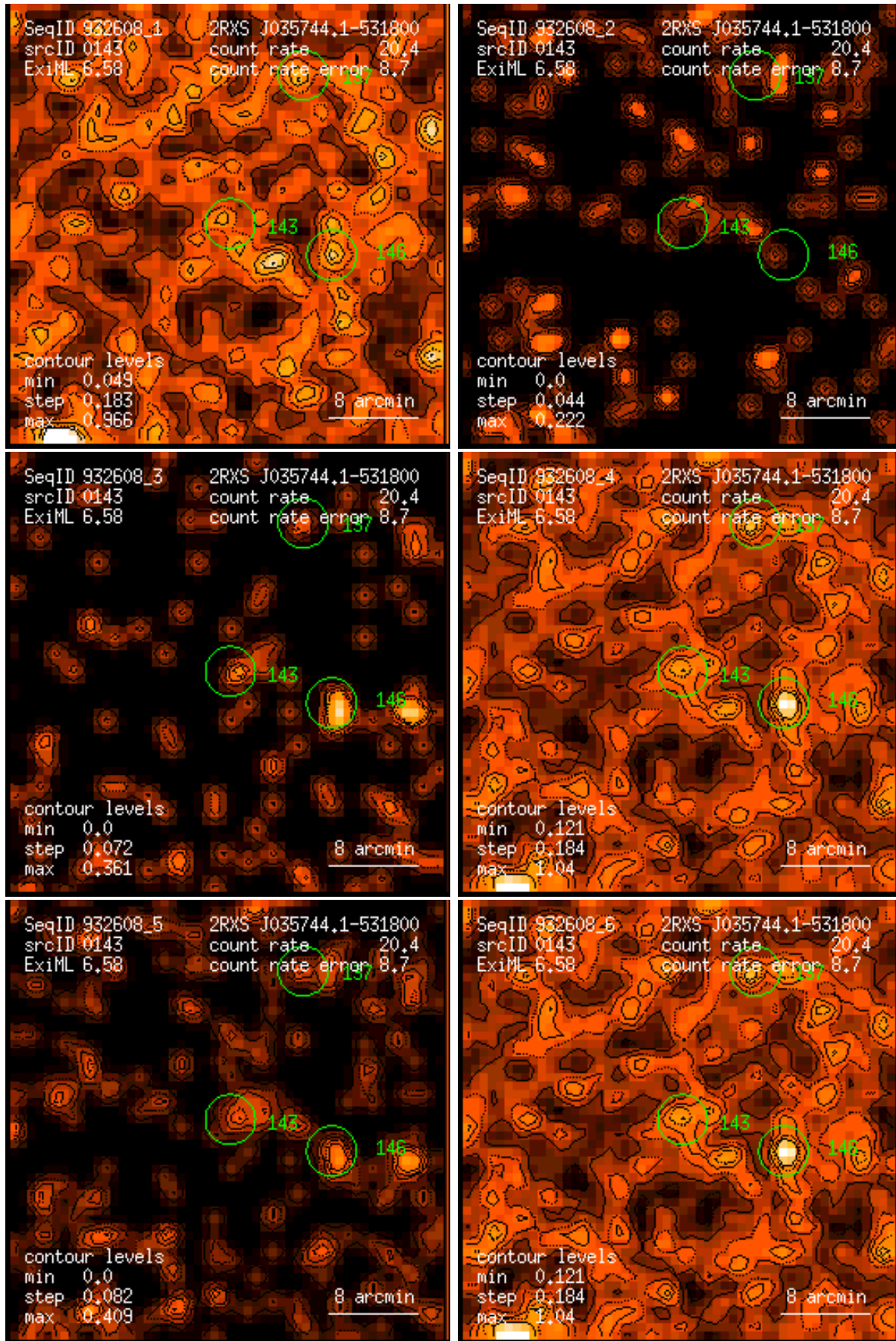
Figure 143: RASS 932608: detection 0143: band rate images, Gaussian filter: (1) PSPC channels 11 – 41, (2) 52 – 90, (3) 91 – 201, (4) 11 – 235, (5) 52 – 201, (6) 11 – 201. Broad band rates in counts/ks. Band rate contour levels in counts/ks/arcmin 2 .
