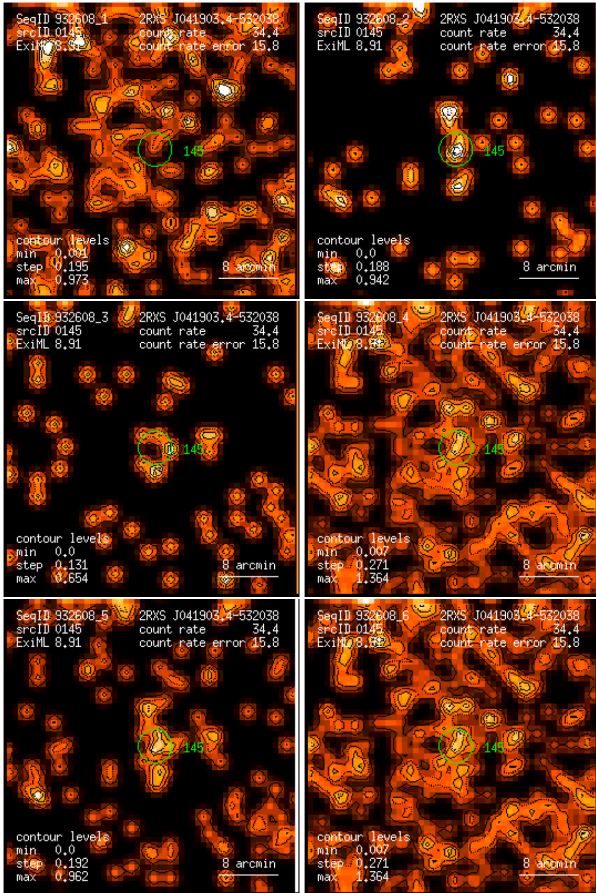
Figure 145: RASS 932608: detection 0145: band rate images, Gaussian filter: (1) PSPC channels 11 – 41, (2) 52 – 90, (3) 91 – 201, (4) 11 – 235, (5) 52 – 201, (6) 11 – 201. Broad band rates in counts/ks. Band rate contour levels in counts/ks/arcmin 2 .
