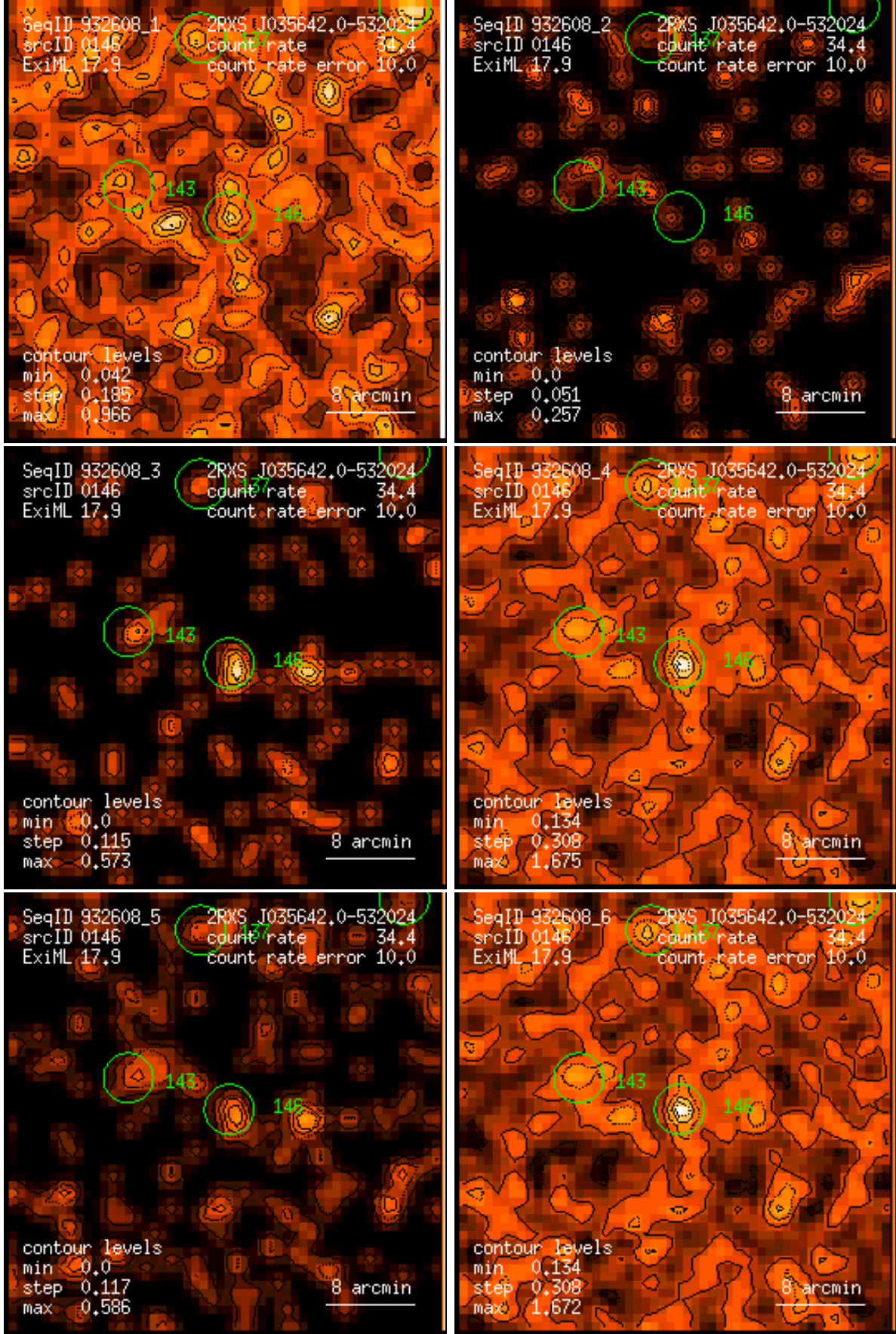
Figure 146: RASS 932608: detection 0146: band rate images, Gaussian filter: (1) PSPC channels 11 – 41, (2) 52 – 90, (3) 91 – 201, (4) 11 – 235, (5) 52 – 201, (6) 11 – 201. Broad band rates in counts/ks. Band rate contour levels in counts/ks/arcmin 2 .
