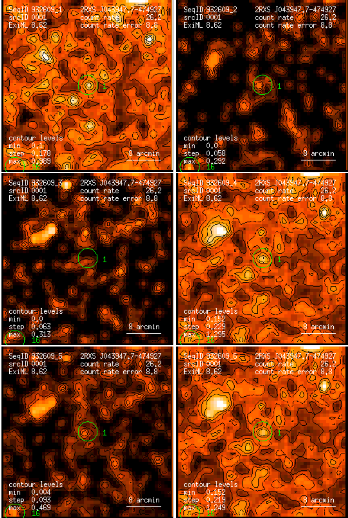
Figure 1: RASS 932609: detection 0001: band rate images, Gaussian filter: (1) PSPC channels 11 – 41, (2) 52 – 90, (3) 91 – 201, (4) 11 – 235, (5) 52 – 201, (6) 11 – 201. Broad band rates in counts/ks. Band rate contour levels in counts/ks/arcmin 2 .
