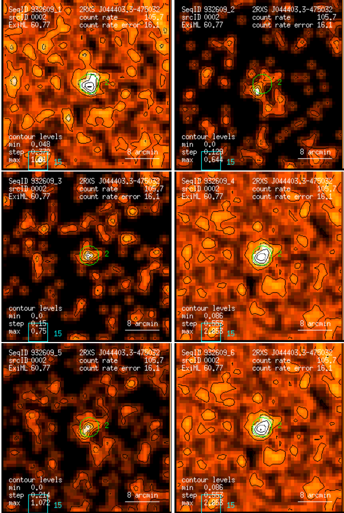
Figure 2: RASS 932609: detection 0002: band rate images, Gaussian filter: (1) PSPC channels 11 – 41, (2) 52 – 90, (3) 91 – 201, (4) 11 – 235, (5) 52 – 201, (6) 11 – 201. Broad band rates in counts/ks. Band rate contour levels in counts/ks/arcmin 2 .
