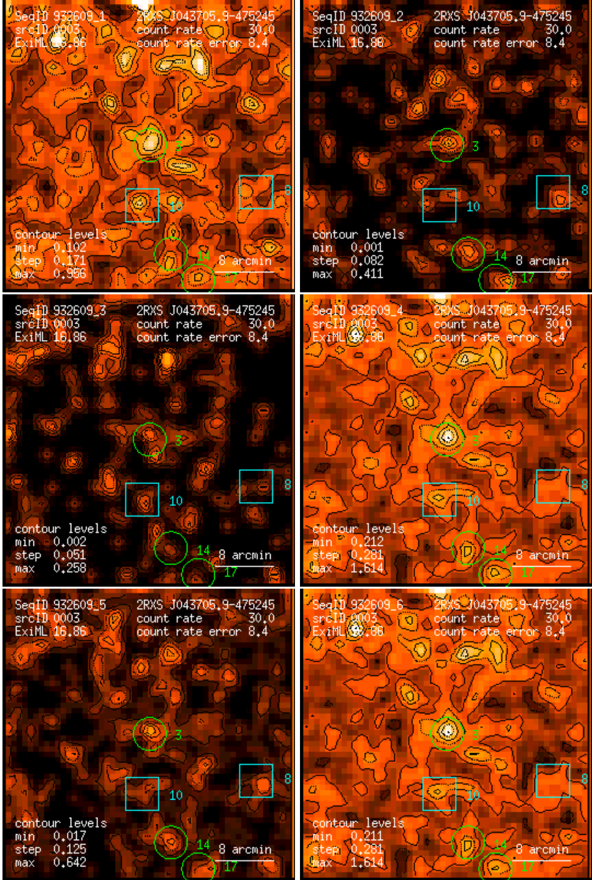
Figure 3: RASS 932609: detection 0003: band rate images, Gaussian filter: (1) PSPC channels 11 – 41, (2) 52 – 90, (3) 91 – 201, (4) 11 – 235, (5) 52 – 201, (6) 11 – 201. Broad band rates in counts/ks. Band rate contour levels in counts/ks/arcmin 2 .
