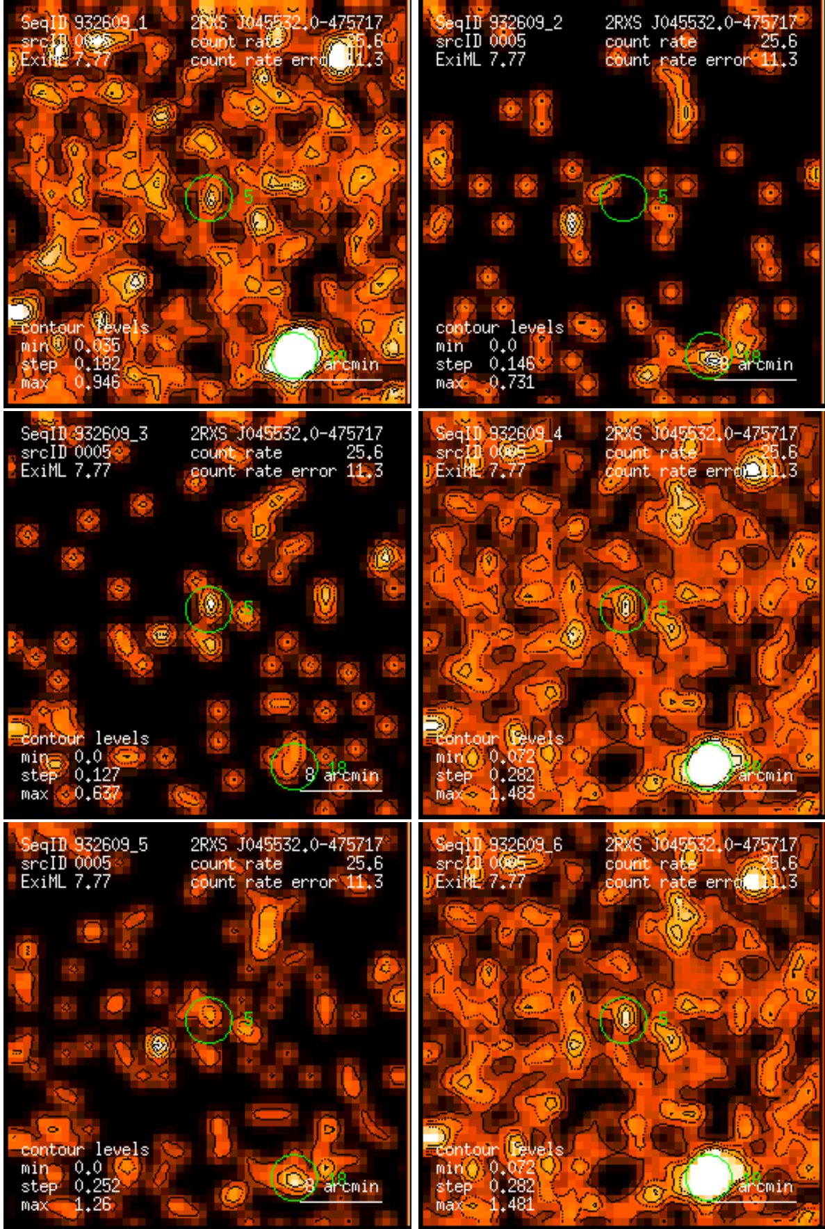
Figure 5: RASS 932609: detection 0005: band rate images, Gaussian filter: (1) PSPC channels 11 – 41, (2) 52 – 90, (3) 91 – 201, (4) 11 – 235, (5) 52 – 201, (6) 11 – 201. Broad band rates in counts/ks. Band rate contour levels in counts/ks/arcmin 2 .
