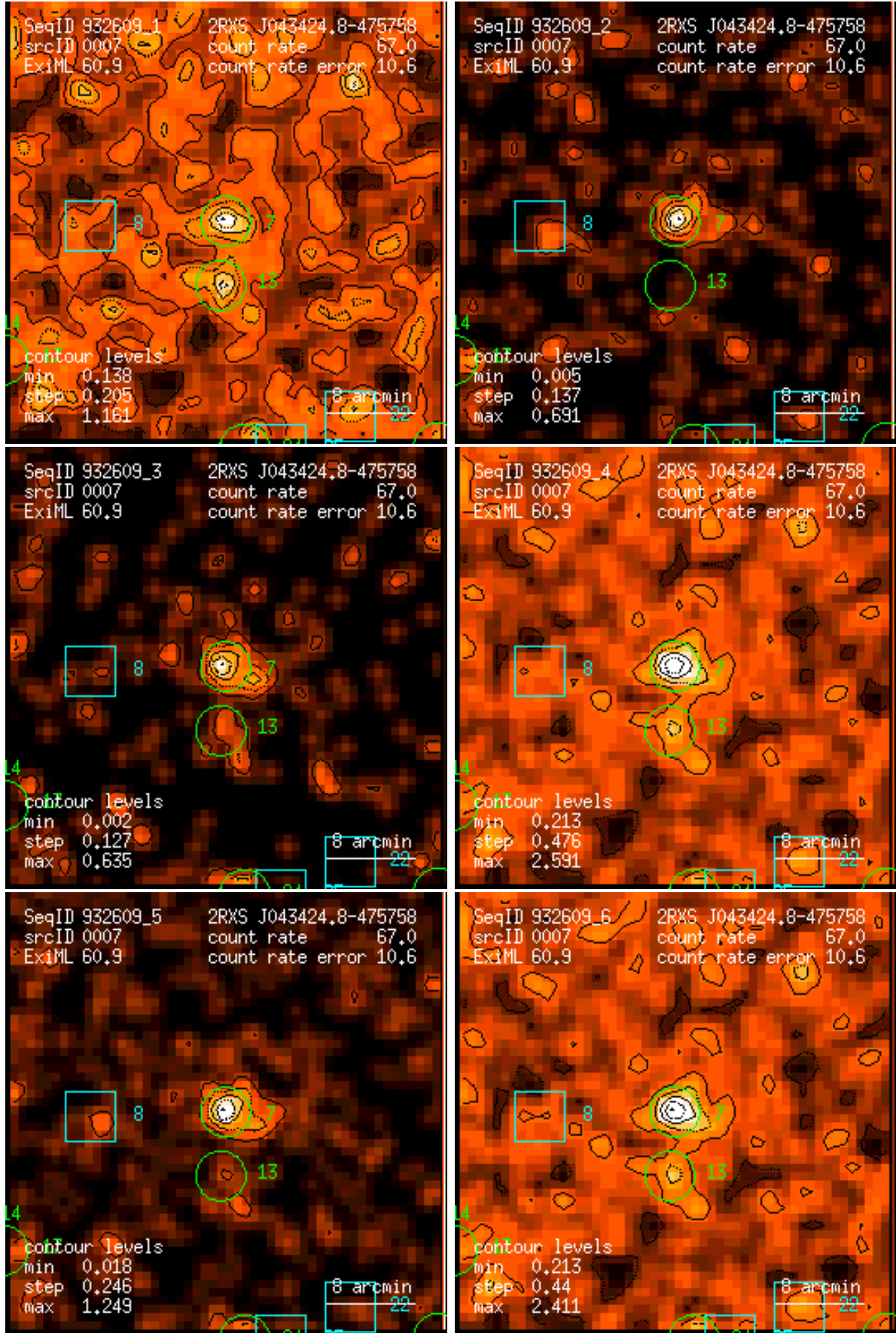
Figure 7: RASS 932609: detection 0007: band rate images, Gaussian filter: (1) PSPC channels 11 – 41, (2) 52 – 90, (3) 91 – 201, (4) 11 – 235, (5) 52 – 201, (6) 11 – 201. Broad band rates in counts/ks. Band rate contour levels in counts/ks/arcmin 2 .
