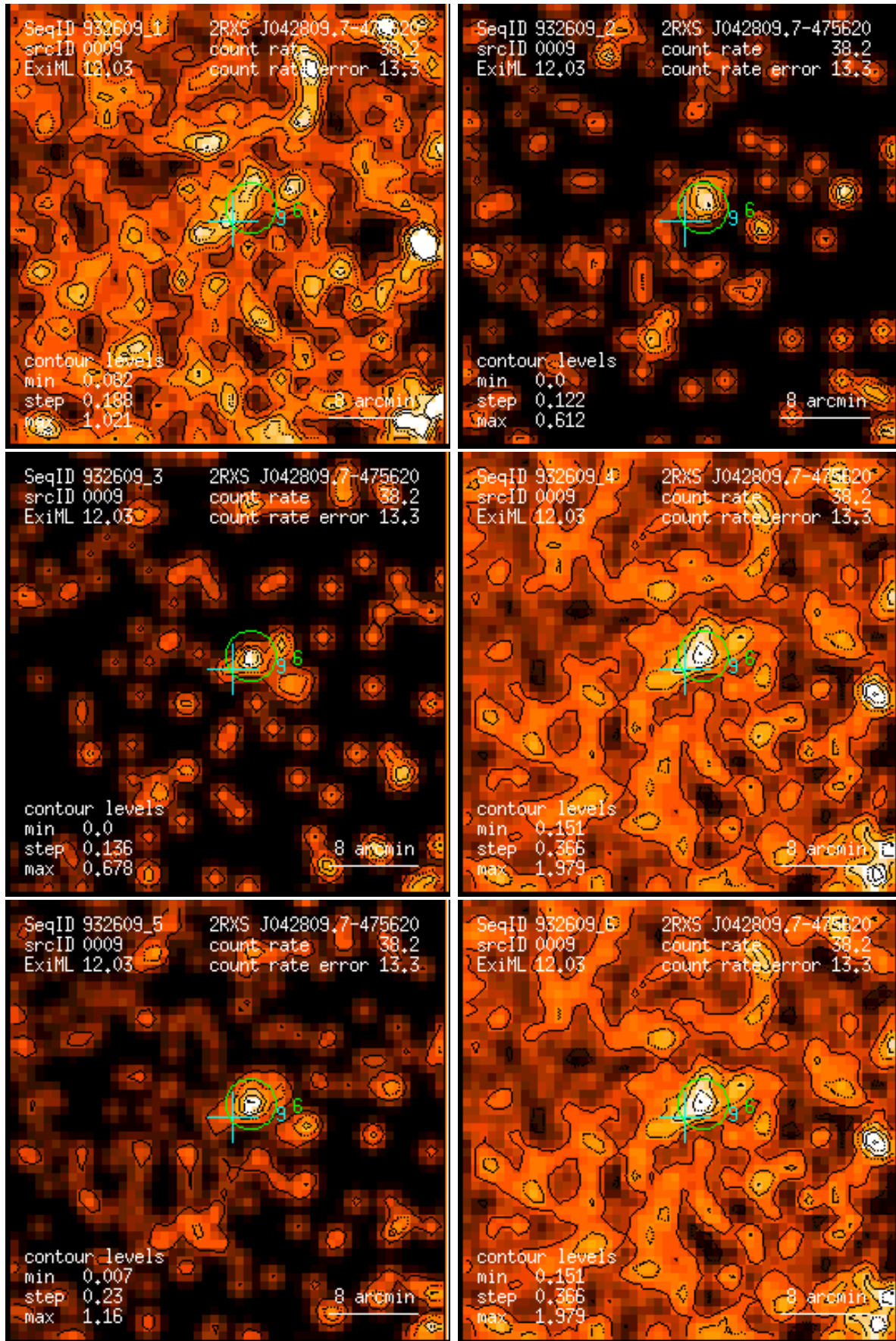
Figure 9: RASS 932609: detection 0009: band rate images, Gaussian filter: (1) PSPC channels 11 – 41, (2) 52 – 90, (3) 91 – 201, (4) 11 – 235, (5) 52 – 201, (6) 11 – 201. Broad band rates in counts/ks. Band rate contour levels in counts/ks/arcmin 2 .
