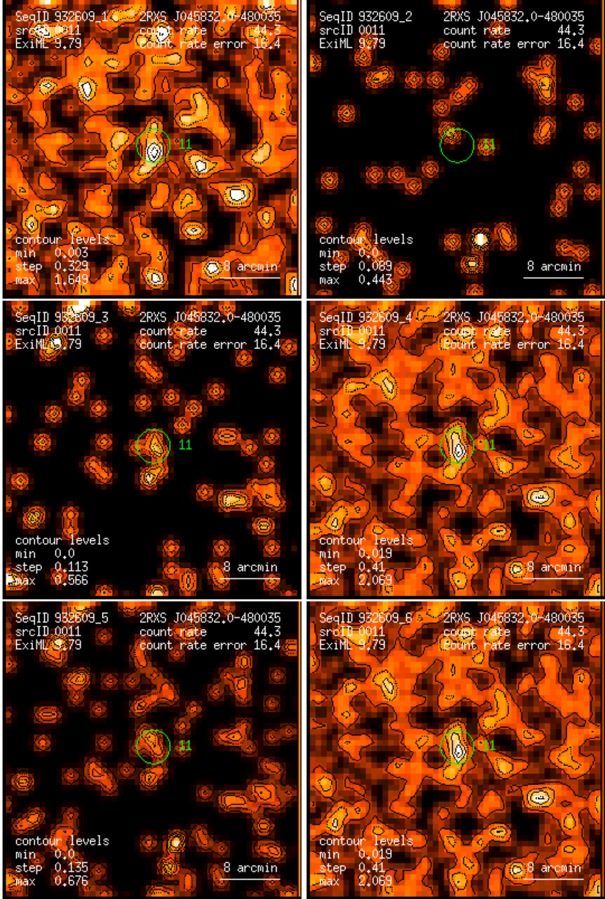
Figure 11: RASS 932609: detection 0011: band rate images, Gaussian filter: (1) PSPC channels 11 – 41, (2) 52 – 90, (3) 91 – 201, (4) 11 – 235, (5) 52 – 201, (6) 11 – 201. Broad band rates in counts/ks. Band rate contour levels in counts/ks/arcmin 2 .
