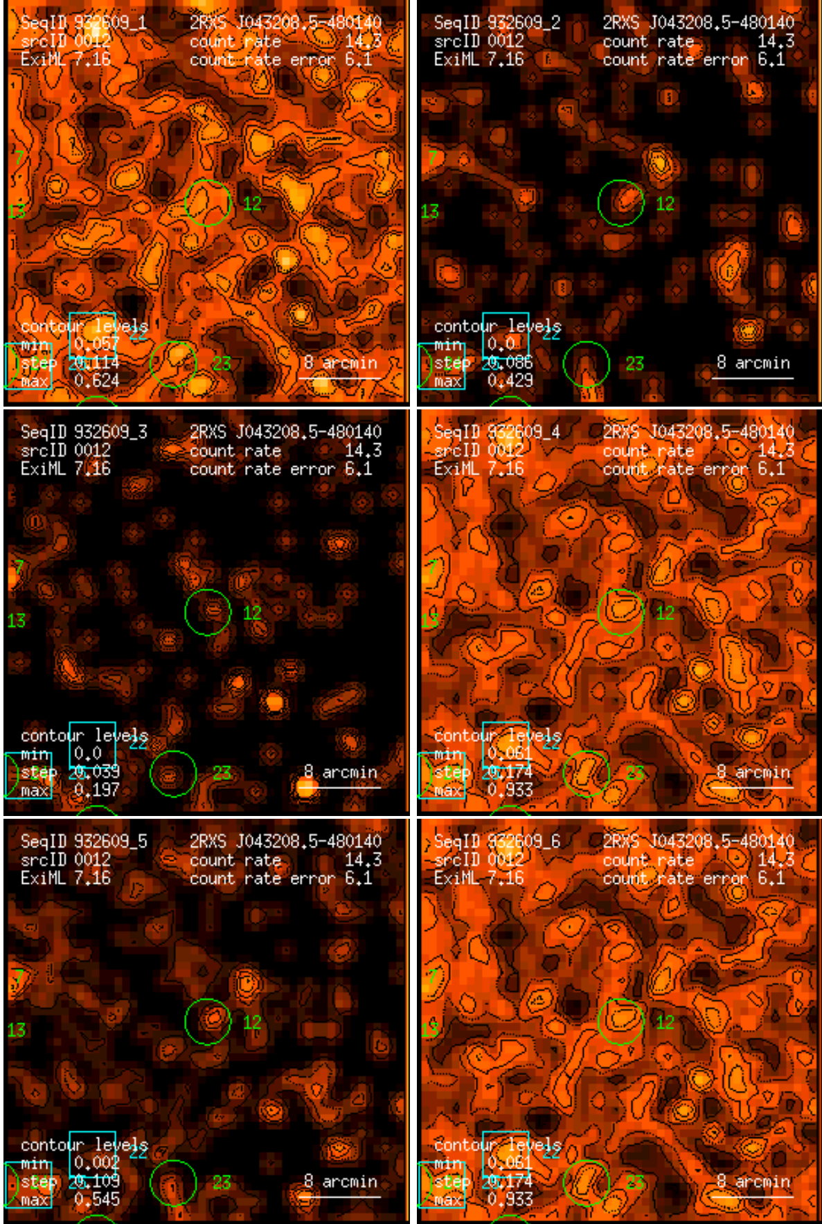
Figure 12: RASS 932609: detection 0012: band rate images, Gaussian filter: (1) PSPC channels 11 – 41, (2) 52 – 90, (3) 91 – 201, (4) 11 – 235, (5) 52 – 201, (6) 11 – 201. Broad band rates in counts/ks. Band rate contour levels in counts/ks/arcmin 2 .
