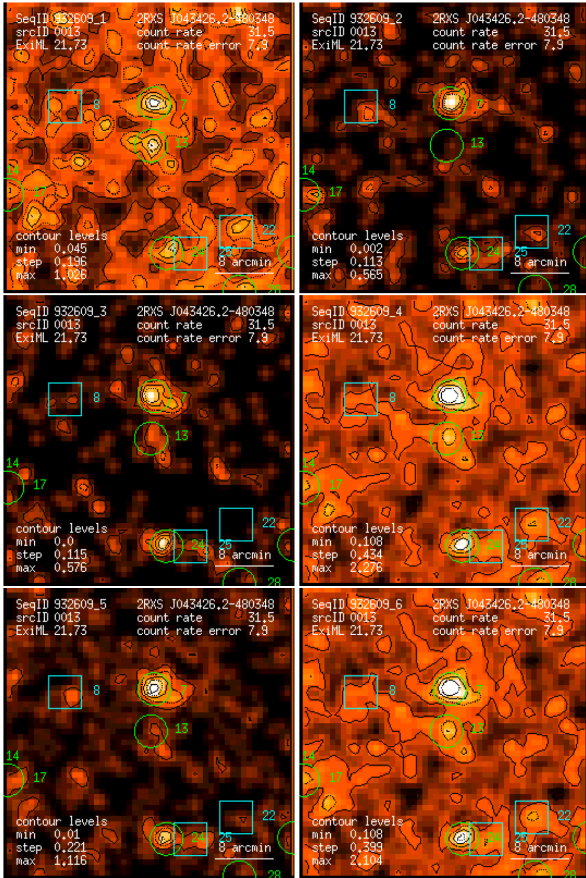
Figure 13: RASS 932609: detection 0013: band rate images, Gaussian filter: (1) PSPC channels 11 – 41, (2) 52 – 90, (3) 91 – 201, (4) 11 – 235, (5) 52 – 201, (6) 11 – 201. Broad band rates in counts/ks. Band rate contour levels in counts/ks/arcmin 2 .
