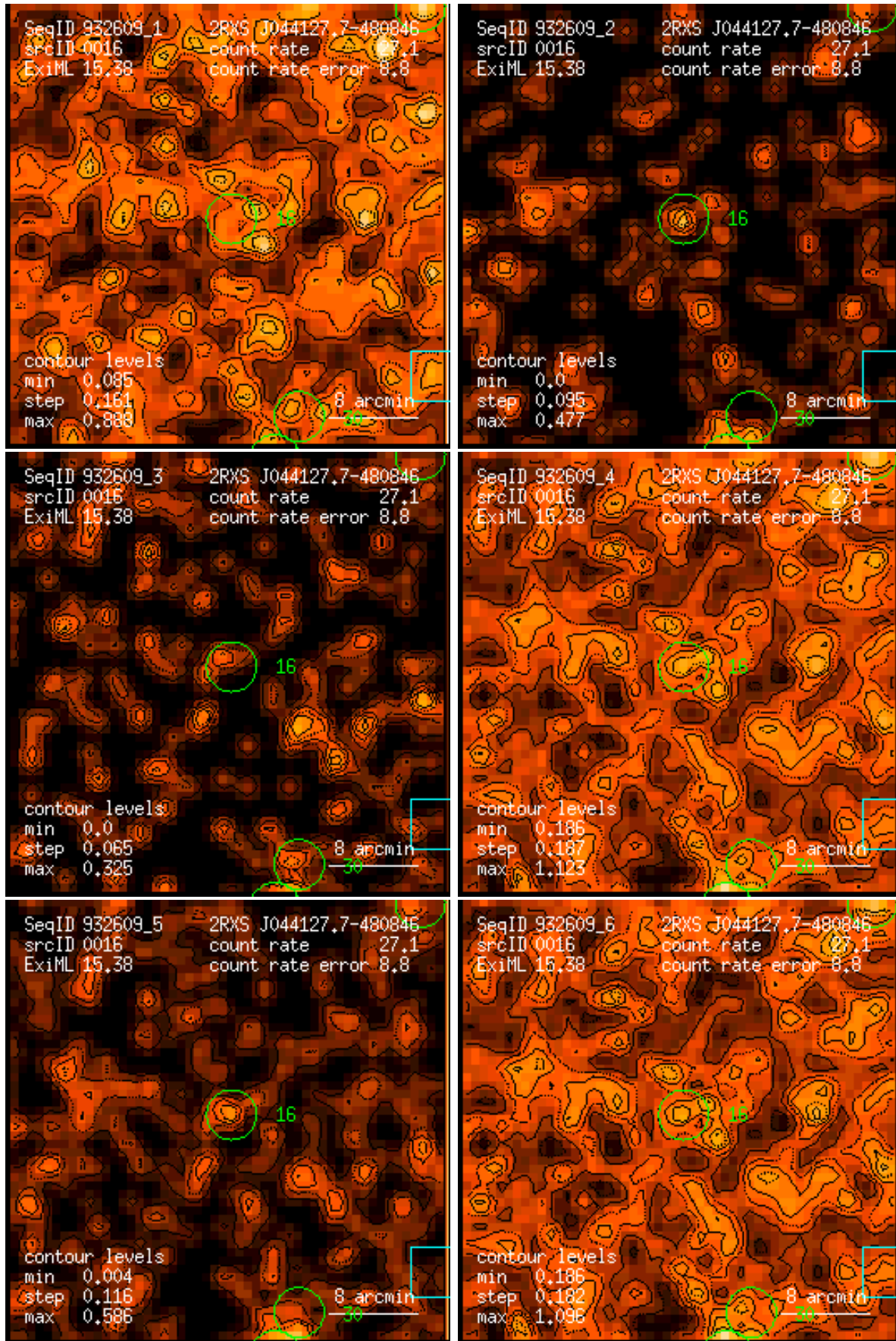
Figure 16: RASS 932609: detection 0016: band rate images, Gaussian filter: (1) PSPC channels 11 – 41, (2) 52 – 90, (3) 91 – 201, (4) 11 – 235, (5) 52 – 201, (6) 11 – 201. Broad band rates in counts/ks. Band rate contour levels in counts/ks/arcmin 2 .
