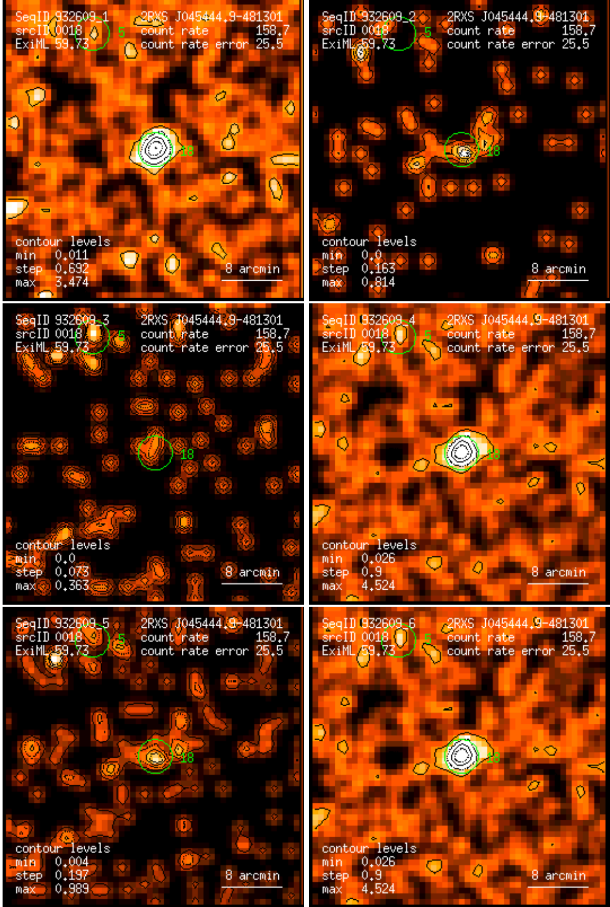
Figure 18: RASS 932609: detection 0018: band rate images, Gaussian filter: (1) PSPC channels 11 – 41, (2) 52 – 90, (3) 91 – 201, (4) 11 – 235, (5) 52 – 201, (6) 11 – 201. Broad band rates in counts/ks. Band rate contour levels in counts/ks/arcmin 2 .
