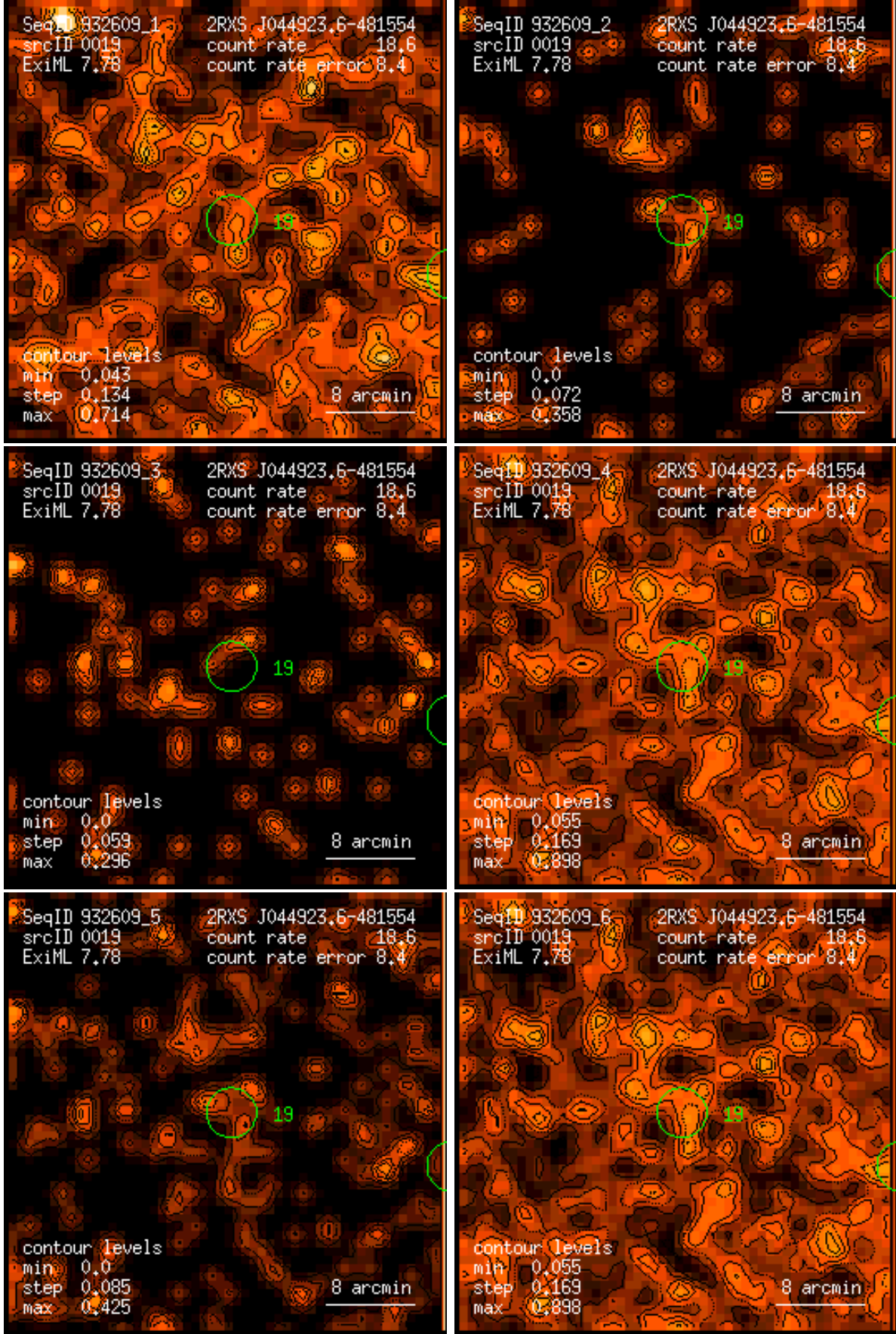
Figure 19: RASS 932609: detection 0019: band rate images, Gaussian filter: (1) PSPC channels 11 – 41, (2) 52 – 90, (3) 91 – 201, (4) 11 – 235, (5) 52 – 201, (6) 11 – 201. Broad band rates in counts/ks. Band rate contour levels in counts/ks/arcmin 2 .
