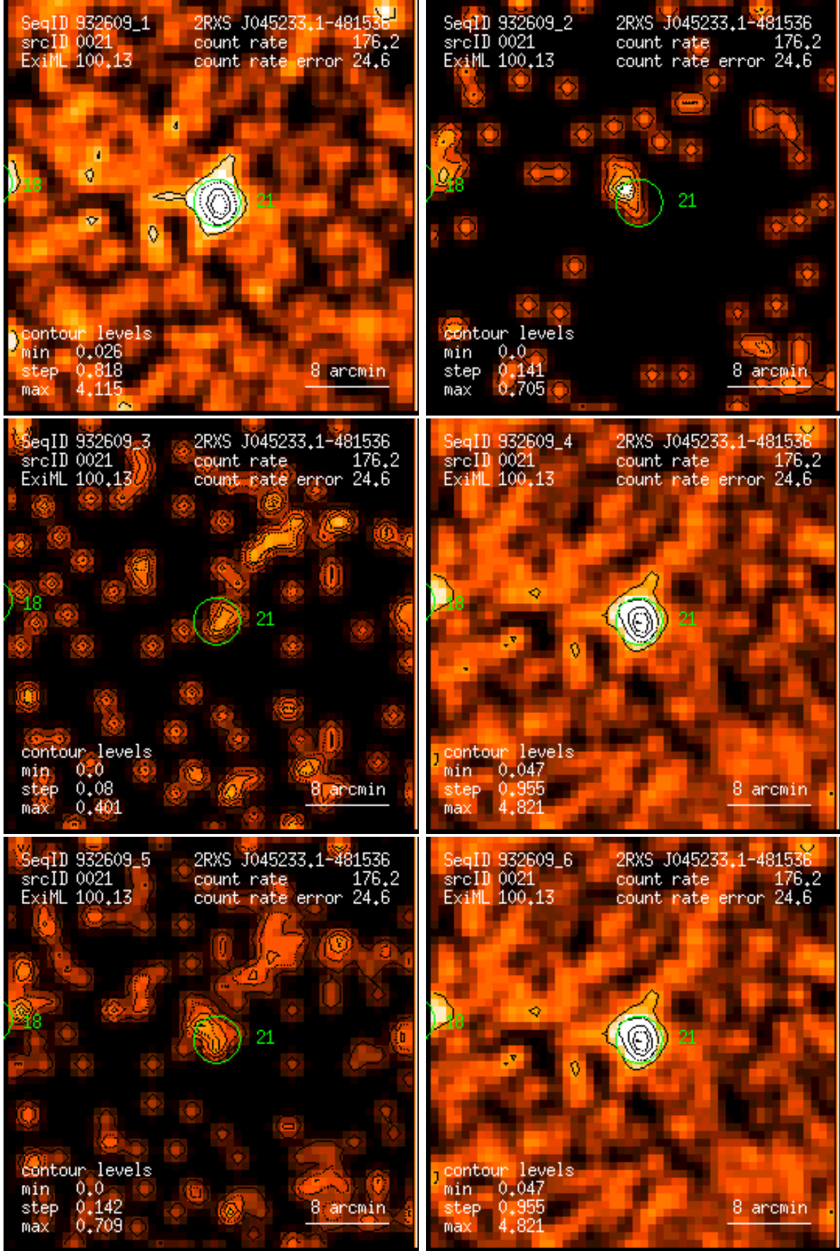
Figure 21: RASS 932609: detection 0021: band rate images, Gaussian filter: (1) PSPC channels 11 – 41, (2) 52 – 90, (3) 91 – 201, (4) 11 – 235, (5) 52 – 201, (6) 11 – 201. Broad band rates in counts/ks. Band rate contour levels in counts/ks/arcmin 2 .
