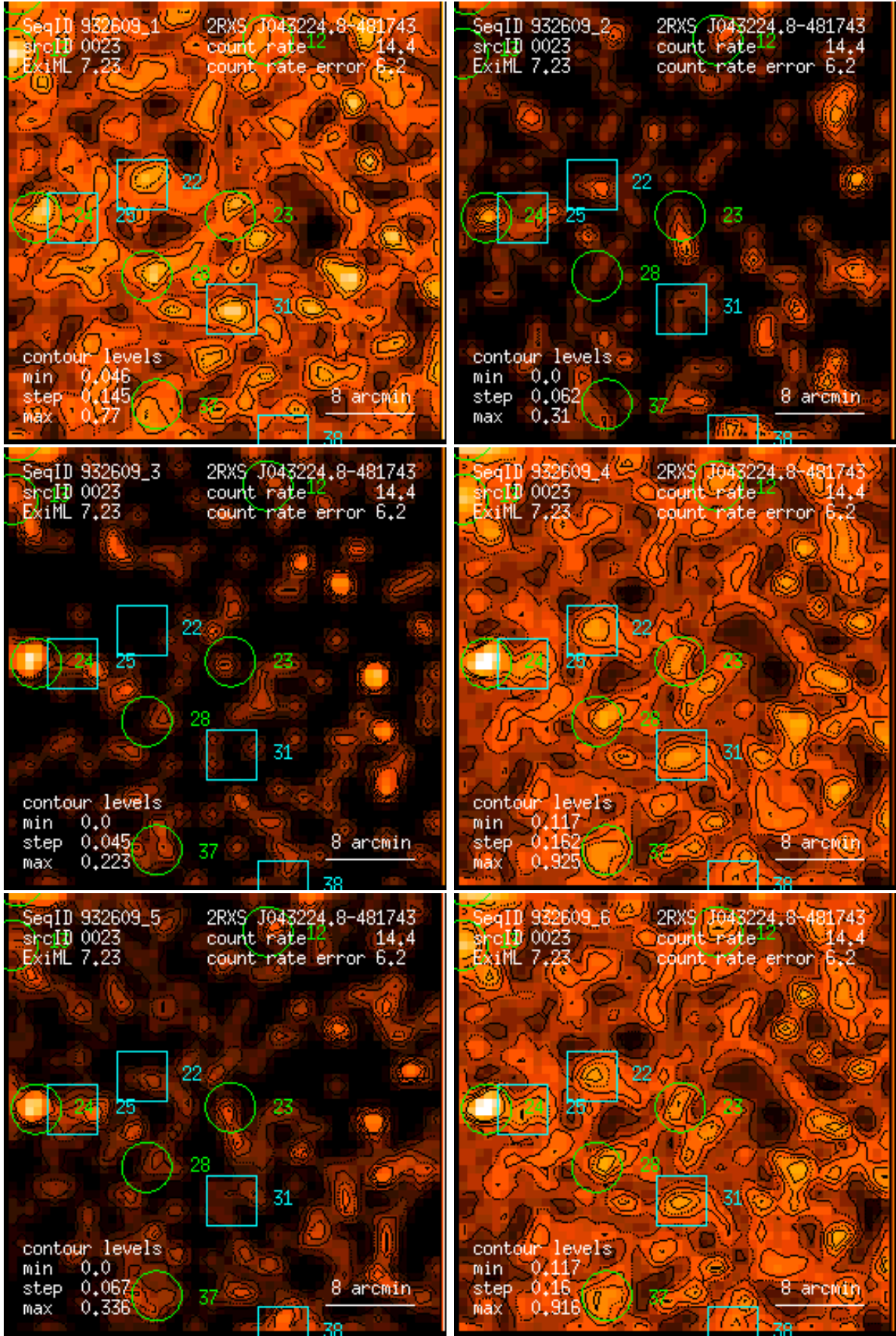
Figure 23: RASS 932609: detection 0023: band rate images, Gaussian filter: (1) PSPC channels 11 – 41, (2) 52 – 90, (3) 91 – 201, (4) 11 – 235, (5) 52 – 201, (6) 11 – 201. Broad band rates in counts/ks. Band rate contour levels in counts/ks/arcmin 2 .
