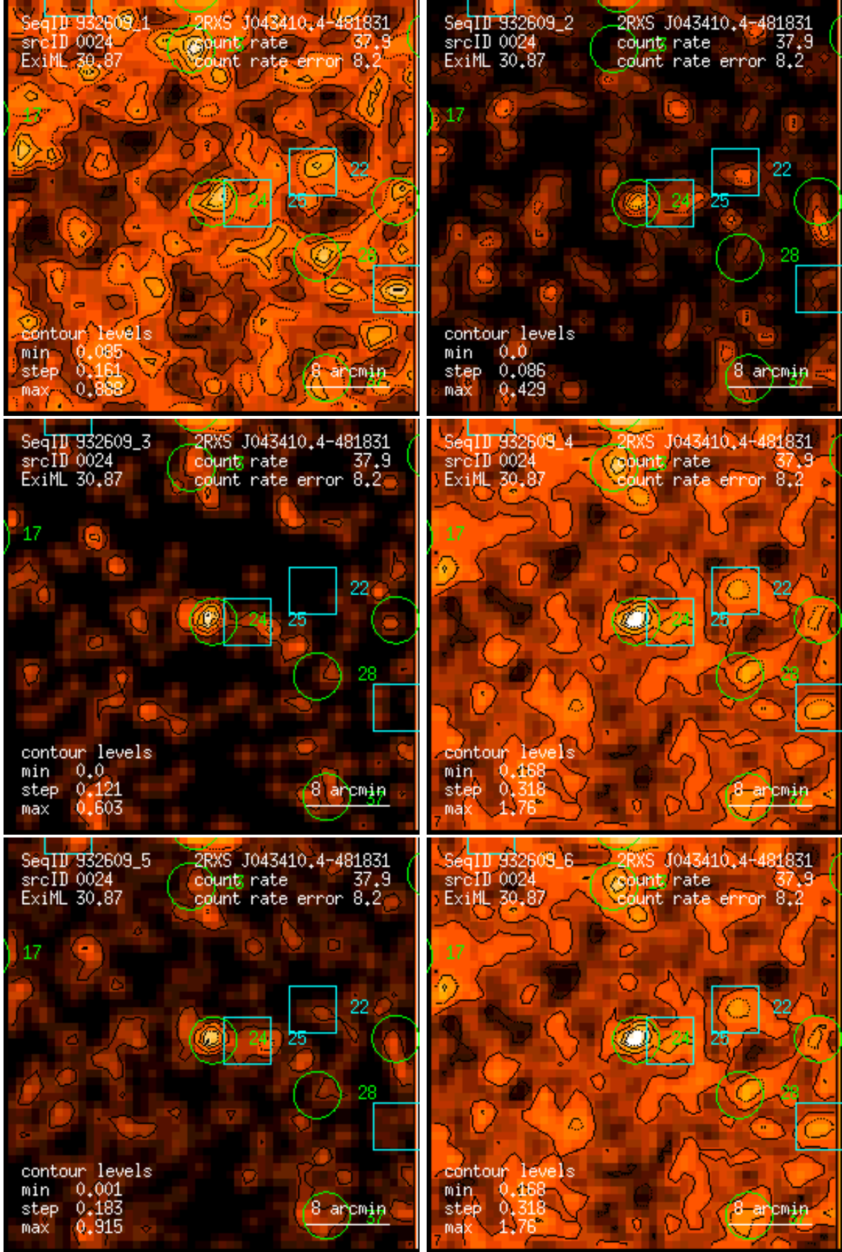
Figure 24: RASS 932609: detection 0024: band rate images, Gaussian filter: (1) PSPC channels 11 – 41, (2) 52 – 90, (3) 91 – 201, (4) 11 – 235, (5) 52 – 201, (6) 11 – 201. Broad band rates in counts/ks. Band rate contour levels in counts/ks/arcmin 2 .
