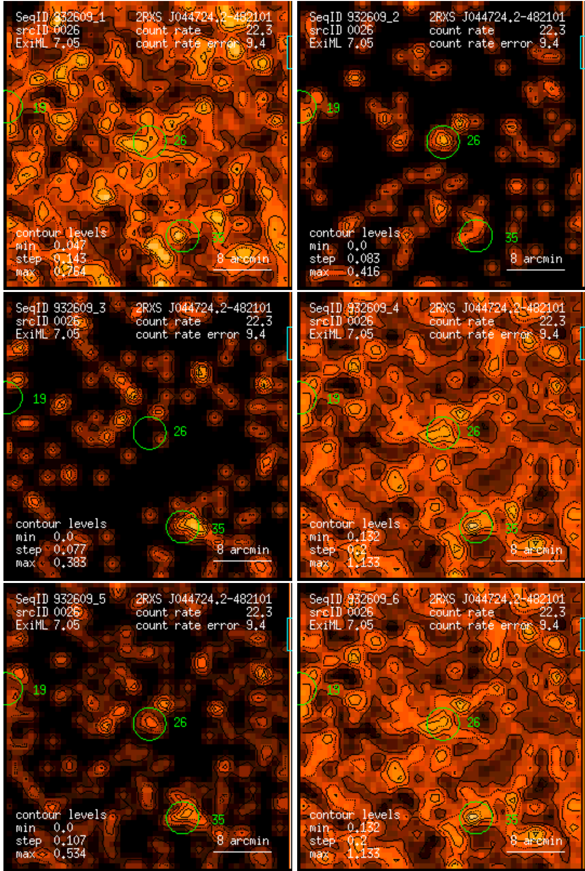
Figure 26: RASS 932609: detection 0026: band rate images, Gaussian filter: (1) PSPC channels 11 – 41, (2) 52 – 90, (3) 91 – 201, (4) 11 – 235, (5) 52 – 201, (6) 11 – 201. Broad band rates in counts/ks. Band rate contour levels in counts/ks/arcmin 2 .
