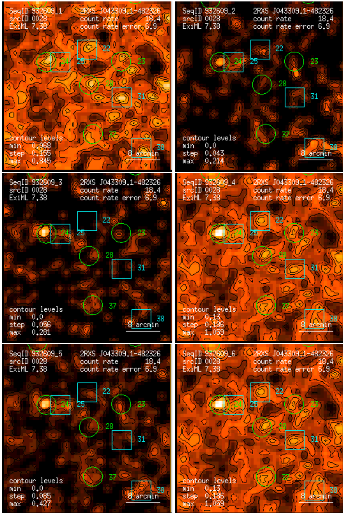
Figure 28: RASS 932609: detection 0028: band rate images, Gaussian filter: (1) PSPC channels 11 – 41, (2) 52 – 90, (3) 91 – 201, (4) 11 – 235, (5) 52 – 201, (6) 11 – 201. Broad band rates in counts/ks. Band rate contour levels in counts/ks/arcmin 2 .
