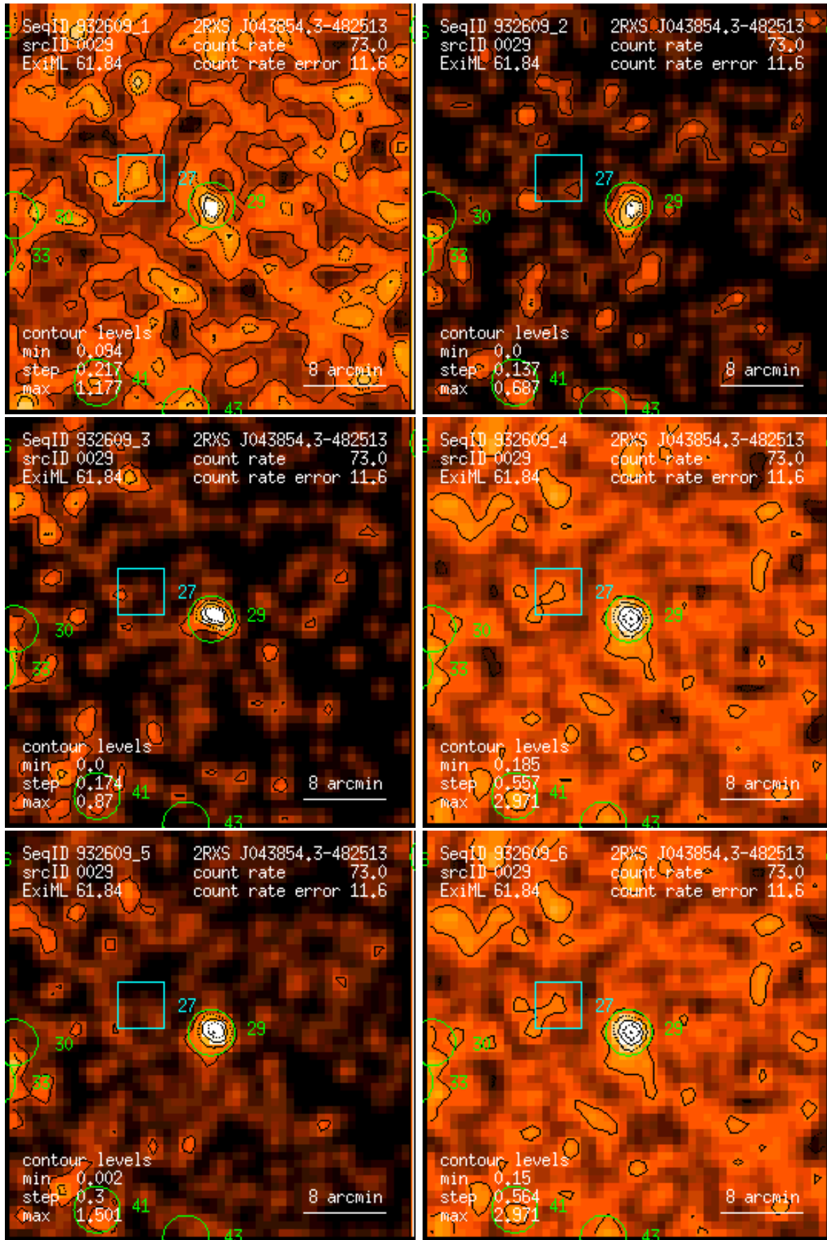
Figure 29: RASS 932609: detection 0029: band rate images, Gaussian filter: (1) PSPC channels 11 – 41, (2) 52 – 90, (3) 91 – 201, (4) 11 – 235, (5) 52 – 201, (6) 11 – 201. Broad band rates in counts/ks. Band rate contour levels in counts/ks/arcmin 2 .
